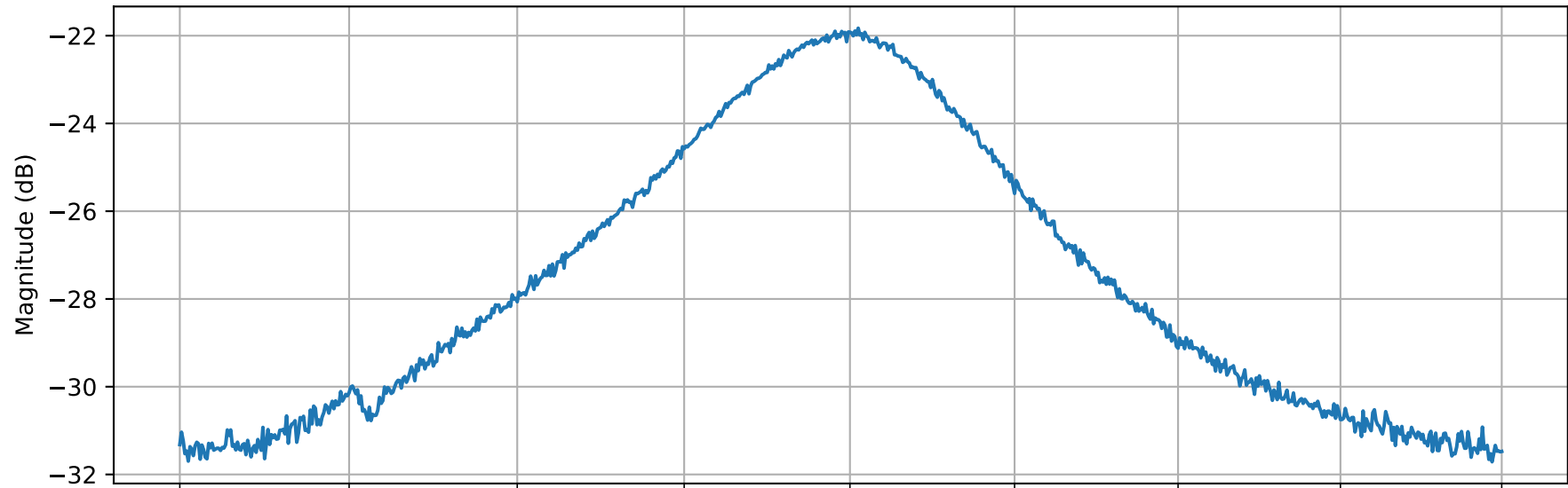
EOM Driver Transfer Function from input to RF Mon - Jan 15 2021 - 16:05:58
