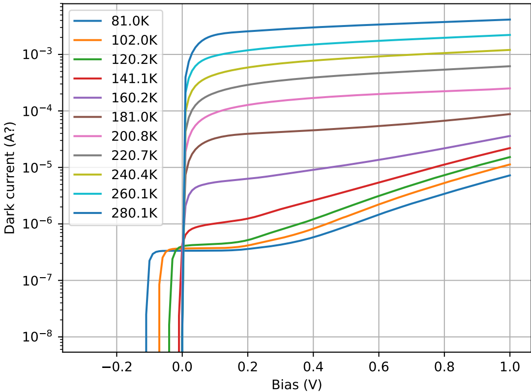
Test3: Dark current vs bias vs temp. Batch 2, diode A1
