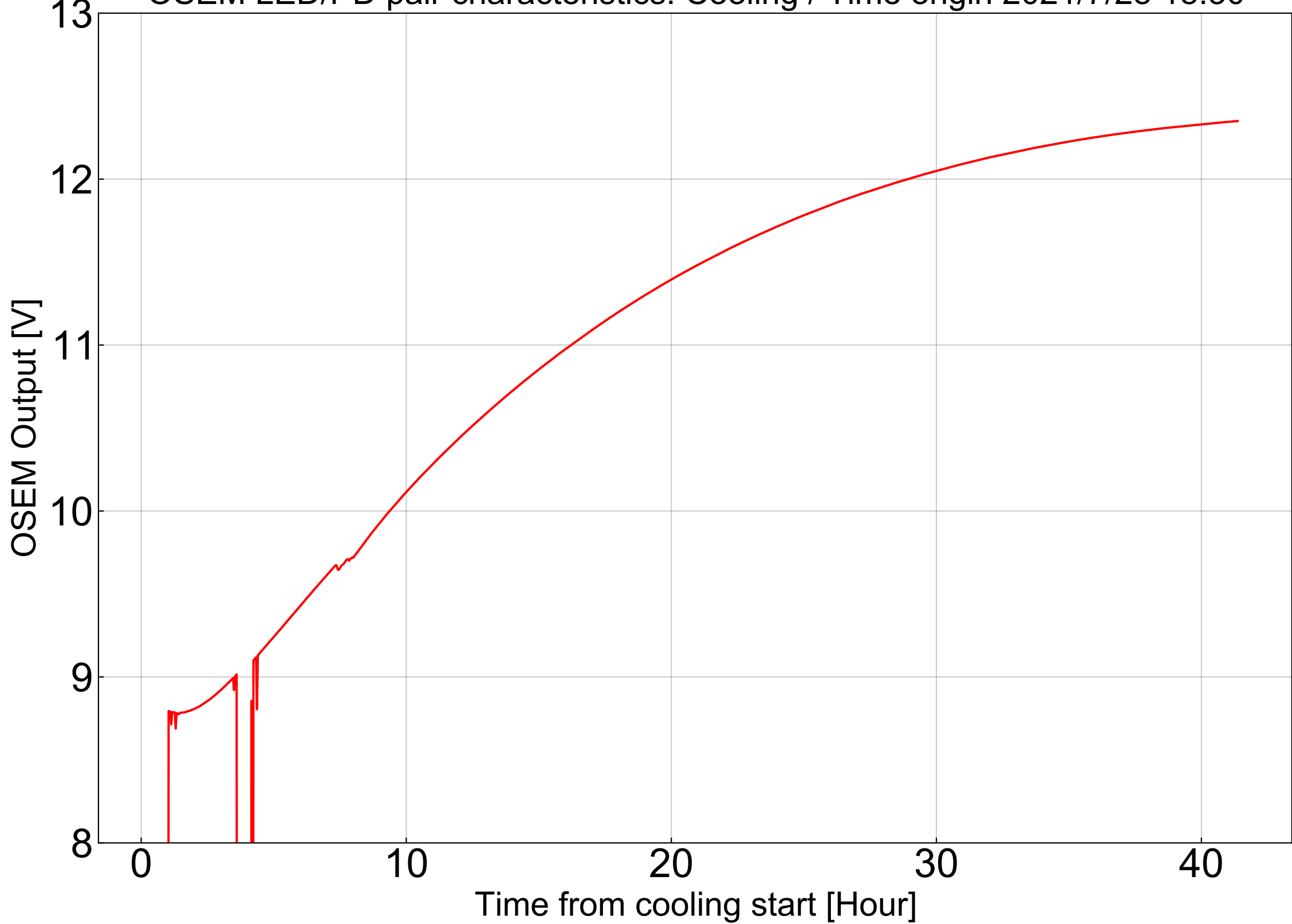
OSEM LED/PD pair characteristics: Cooling / Time origin 2021/7/28 18:30
