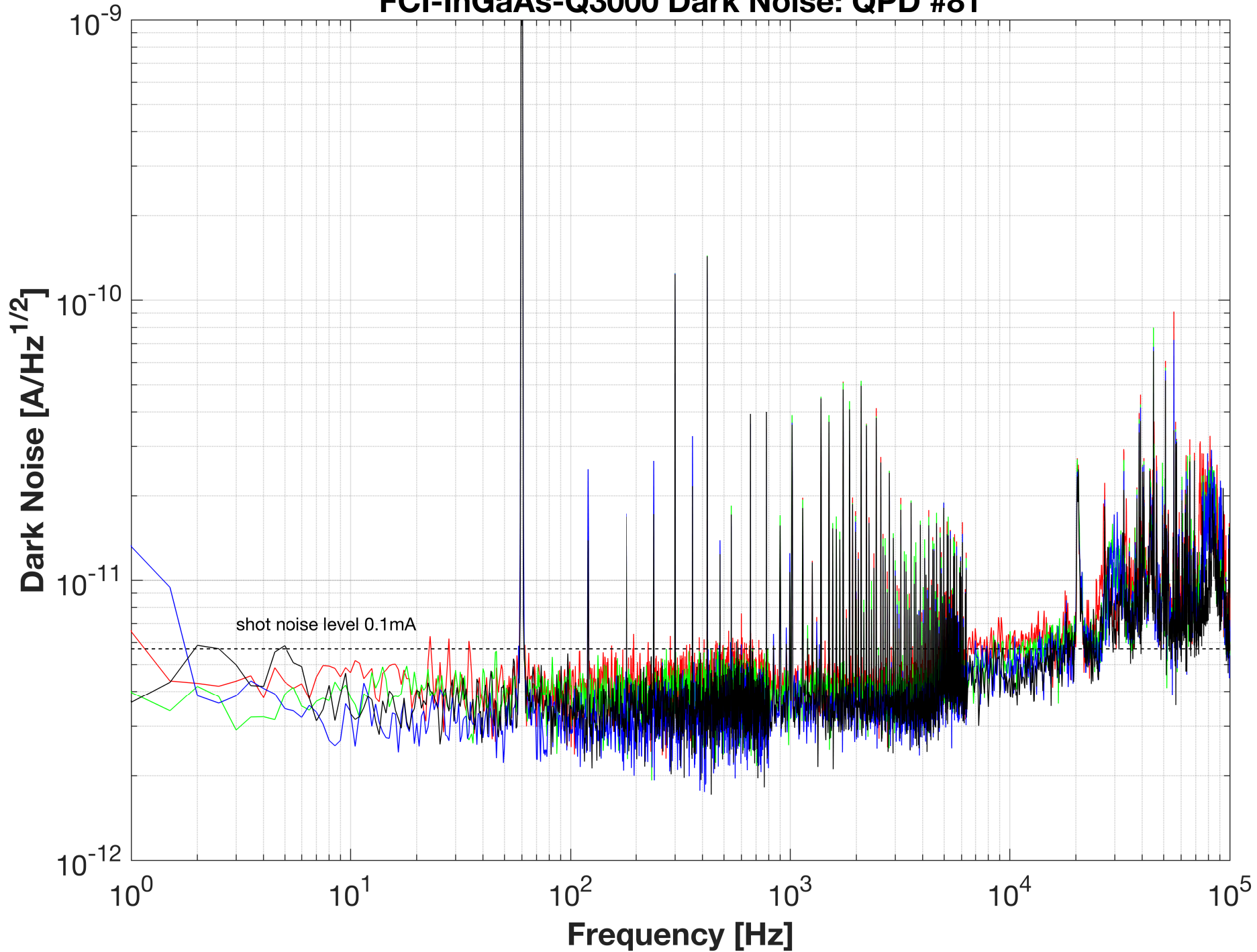
FCI-InGaAs-Q3000 Dark Noise: QPD #81
