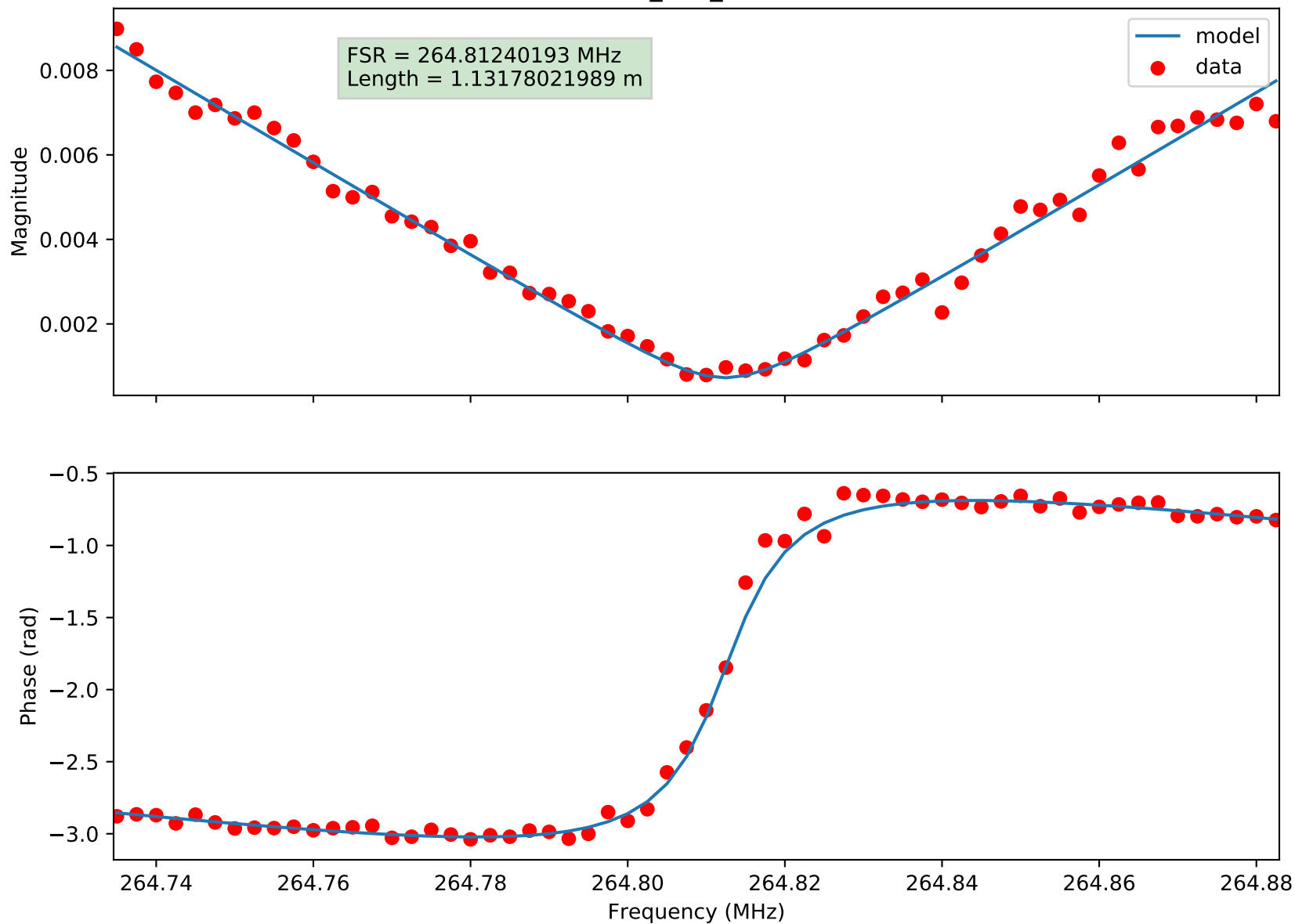
20190423-cavity_alignment Plot of 20190423_FSR_measurement.DAT
