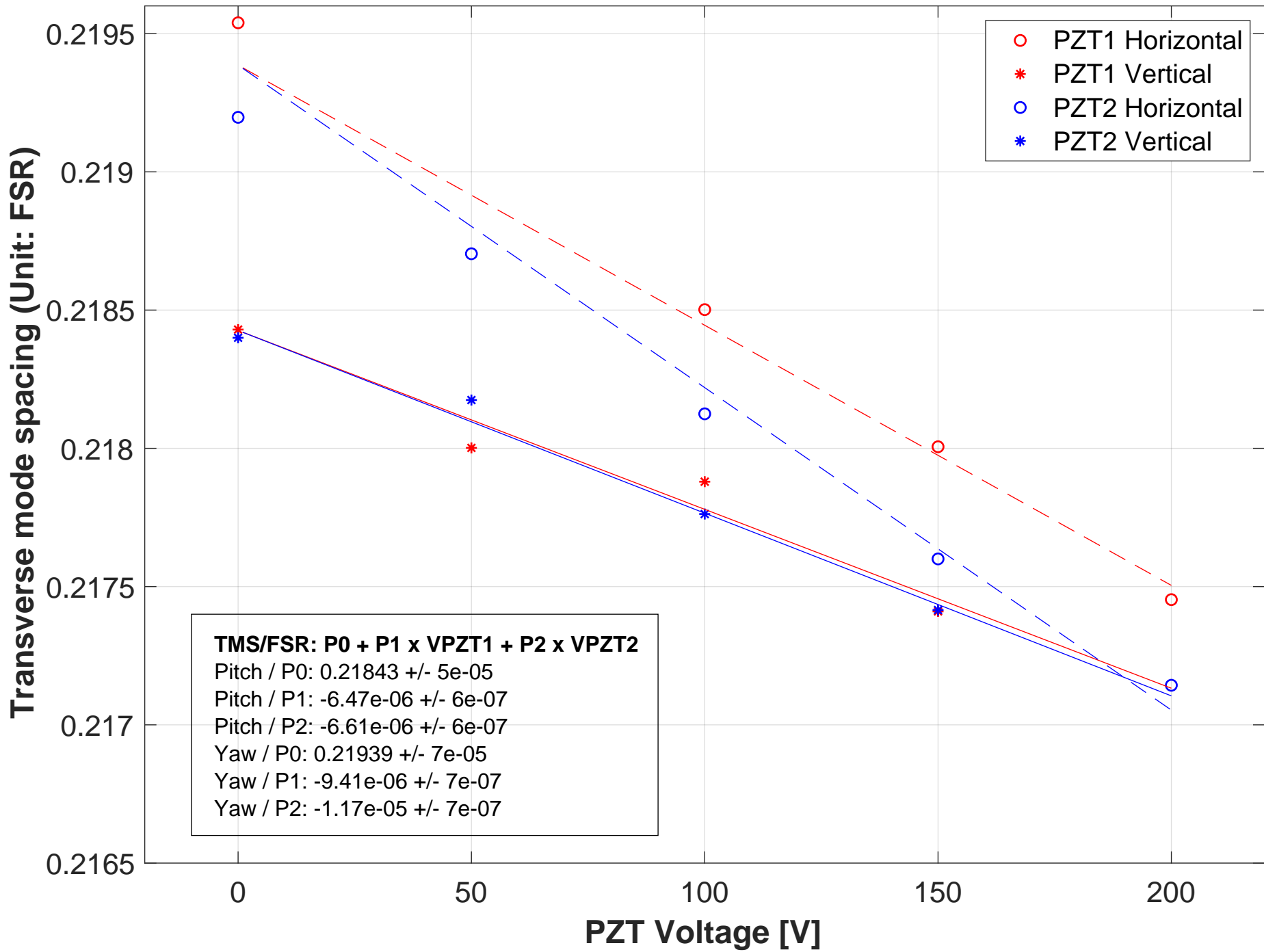
Transverse mode spacing dependence on the PZT voltage
