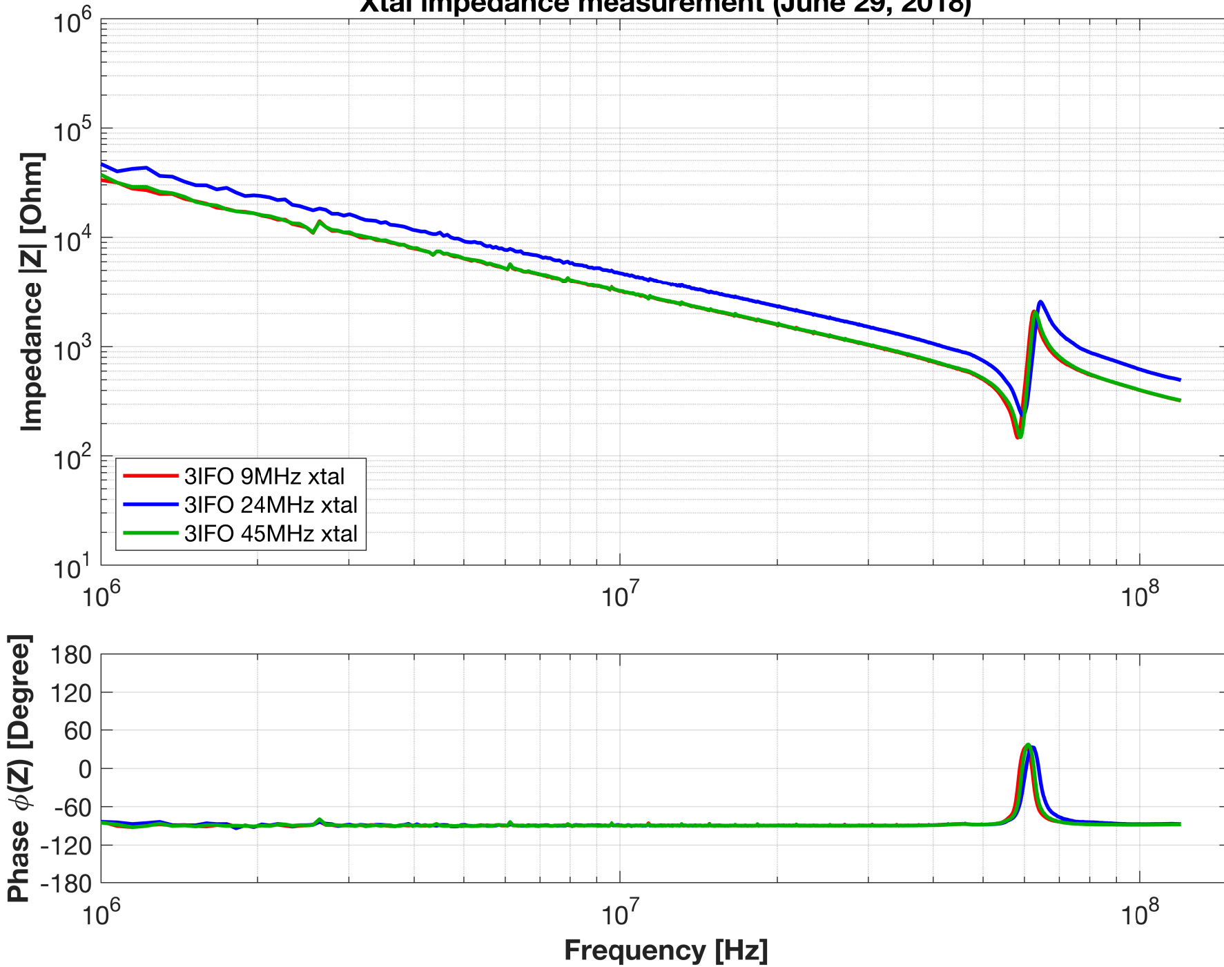
Xtal impedance measurement (June 29, 2018)
