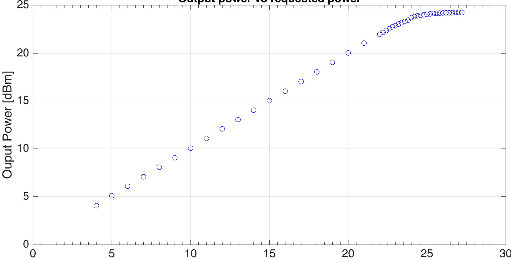
Output power vs requested power
