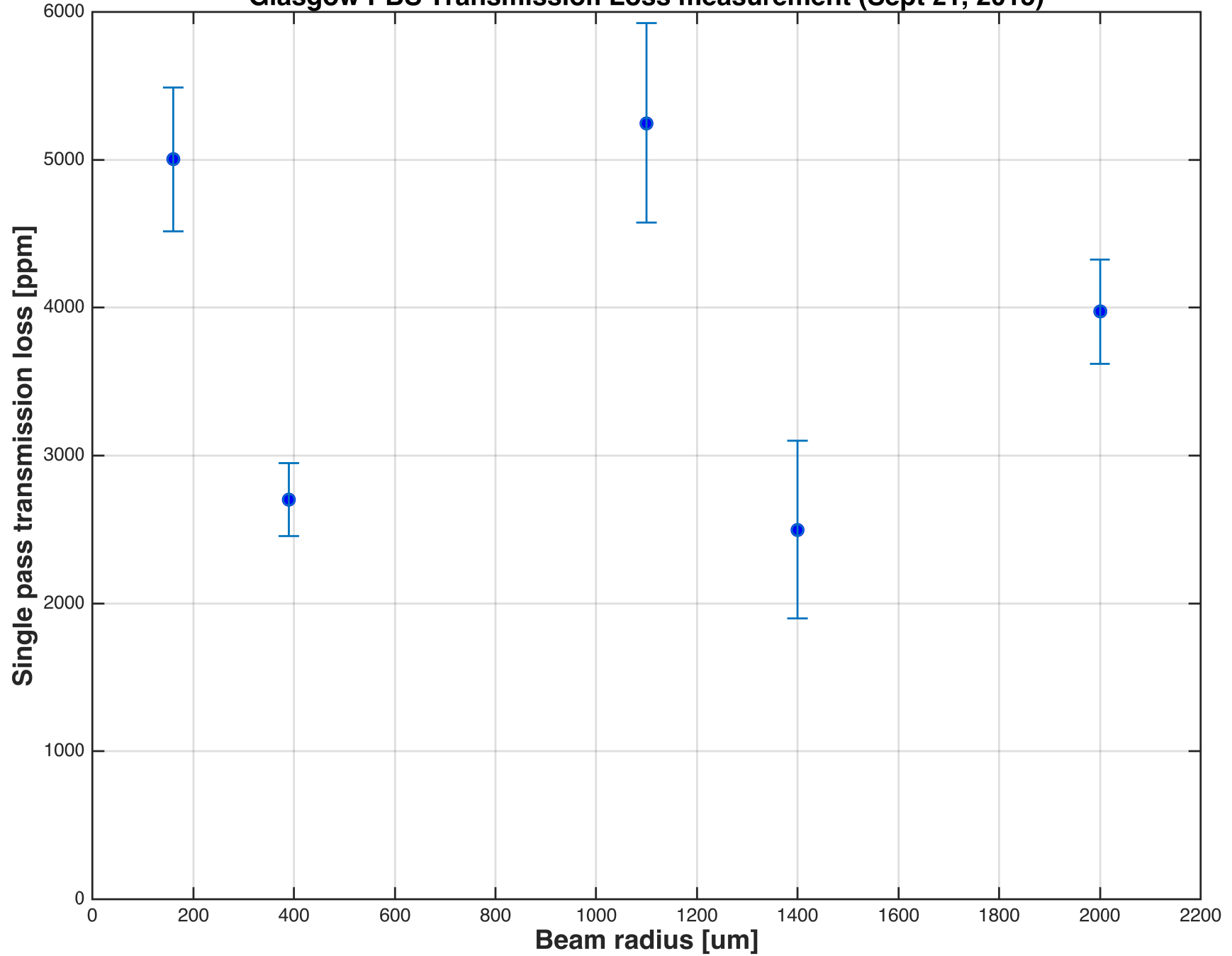
Glasgow PBS Transmission Loss measurement (Sept 21, 2015)
