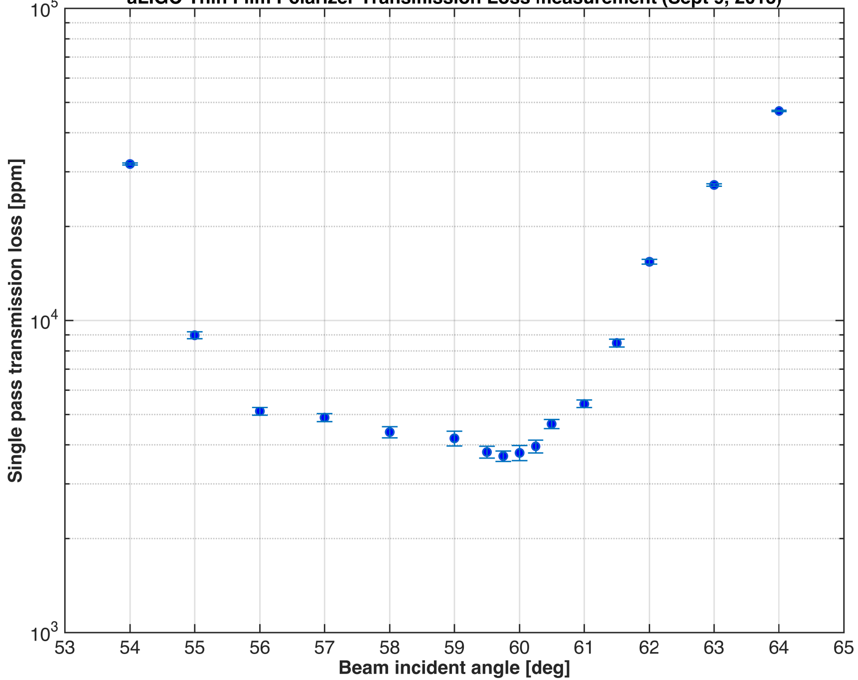
aLIGO Thin Film Polarizer Transmission Loss measurement (Sept 9, 2015)
