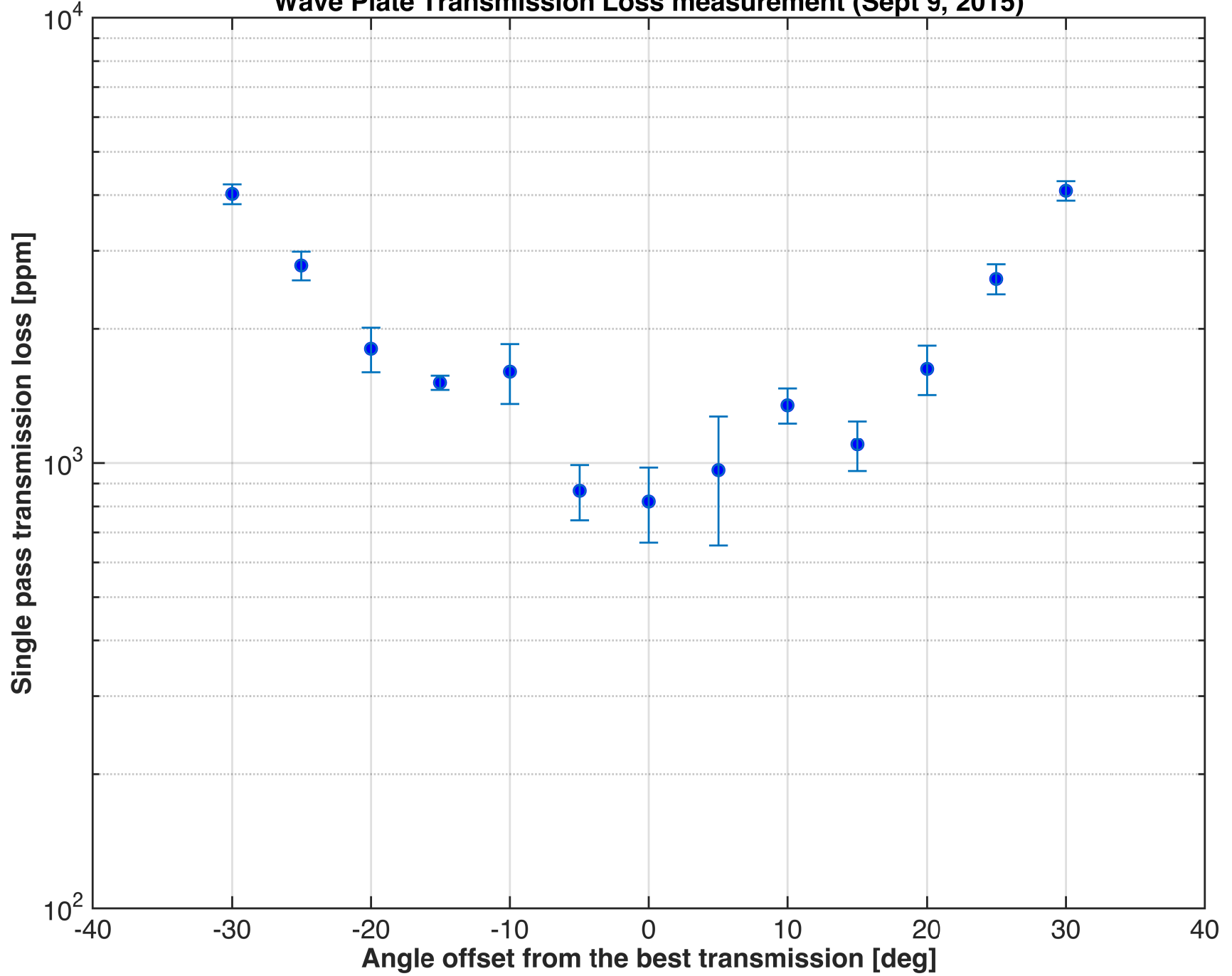
Wave Plate Transmission Loss measurement (Sept 9, 2015)
