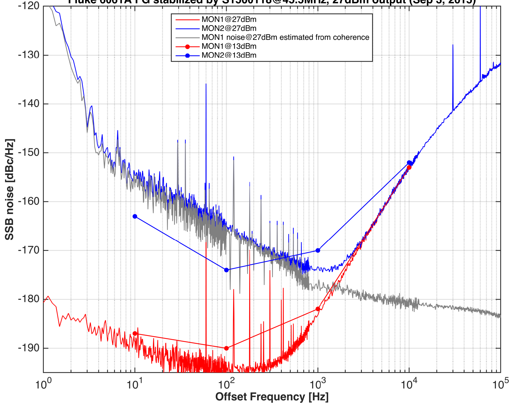
Fluke 6061A FG stabilized by S1500118@45.5MHz, 27dBm output (Sep 3, 2015)
