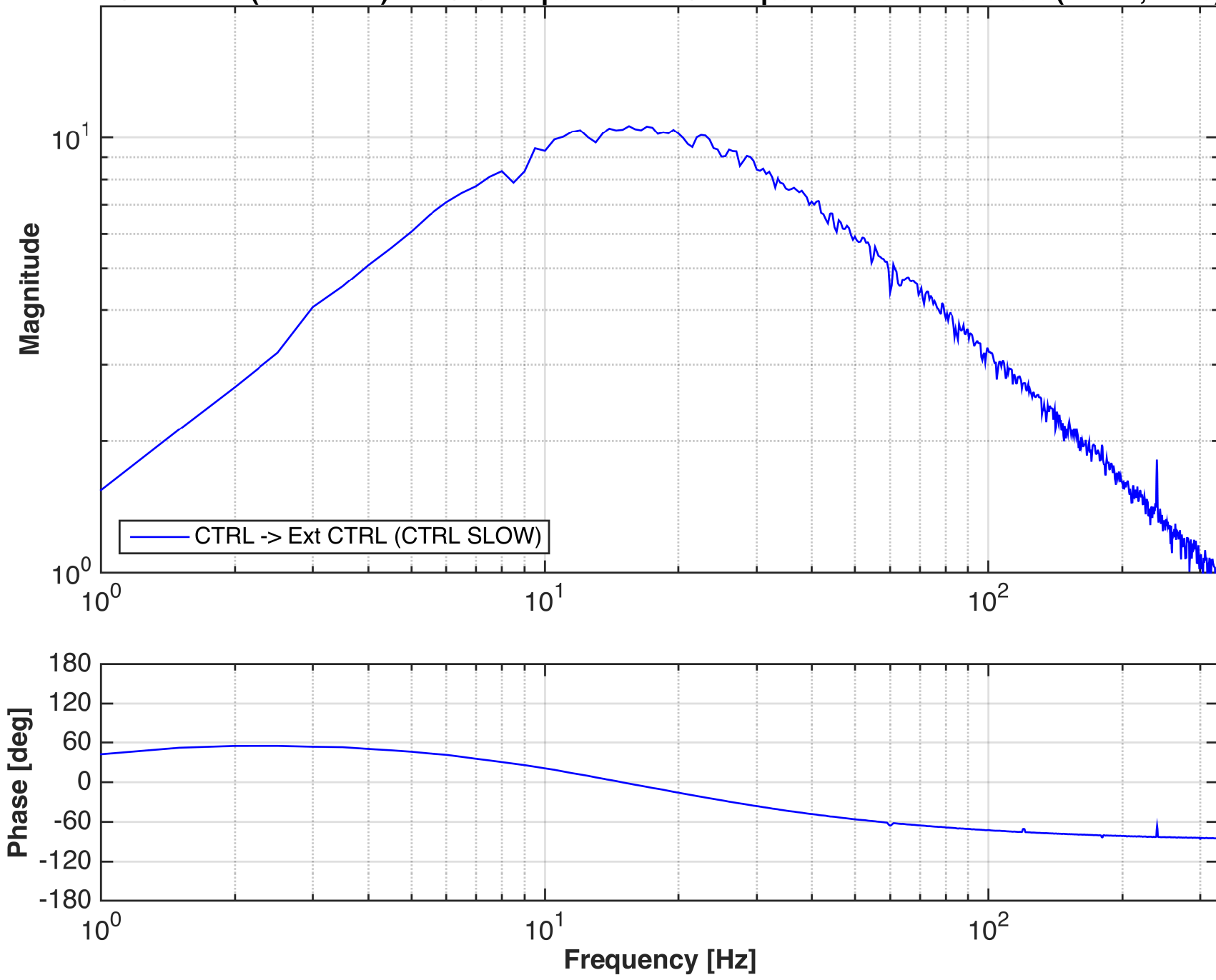
EOM Driver (S1500117): BNC CTRL port -> Ext CTRL port Transfer Function (Jul 22, 2015)
