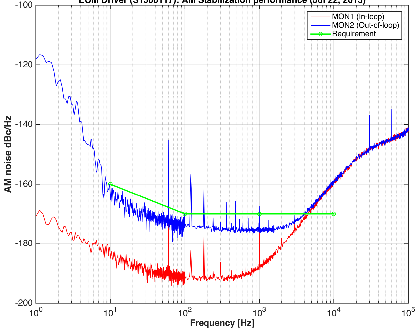
EOM Driver (S1500117): AM Stabilization performance (Jul 22, 2015)
