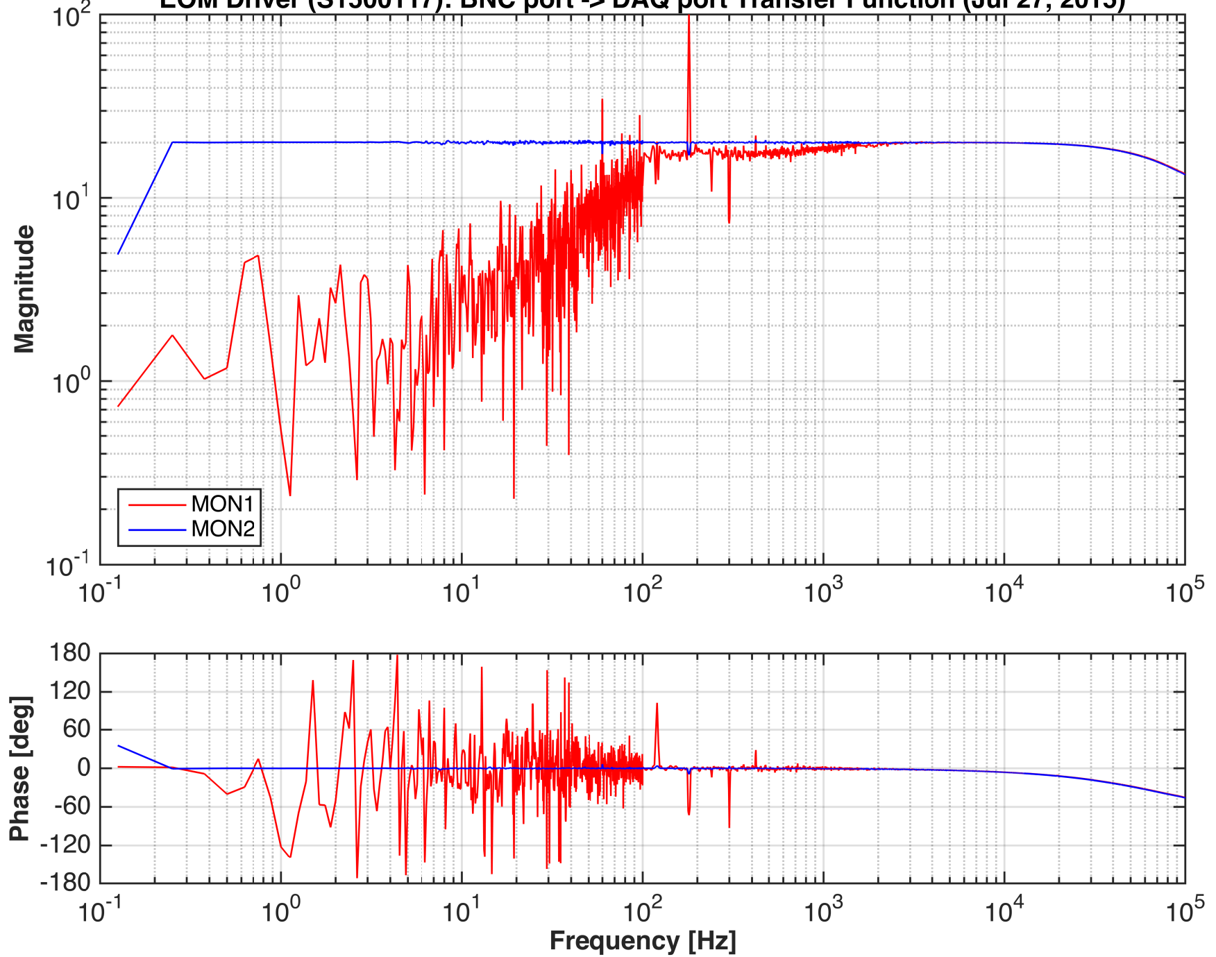
EOM Driver (S1500117): BNC port -> DAQ port Transfer Function (Jul 27, 2015)
