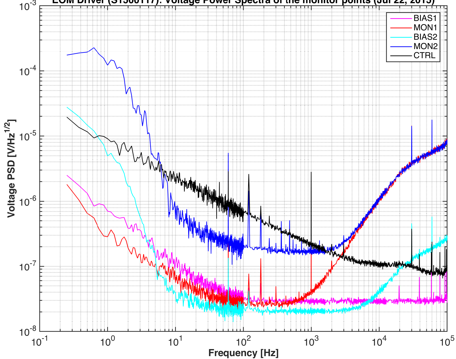
EOM Driver (S1500117): Voltage Power Spectra of the monitor points (Jul 22, 2015)
