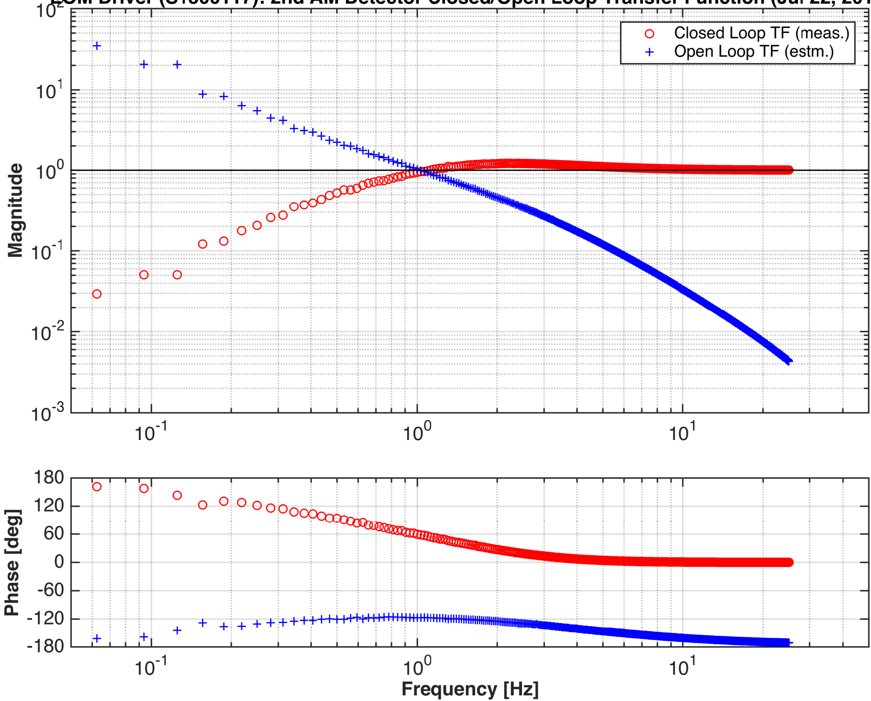
EOM Driver (S1500117): 2nd AM Detector Closed/Open Loop Transfer Function (Jul 22, 2015)
