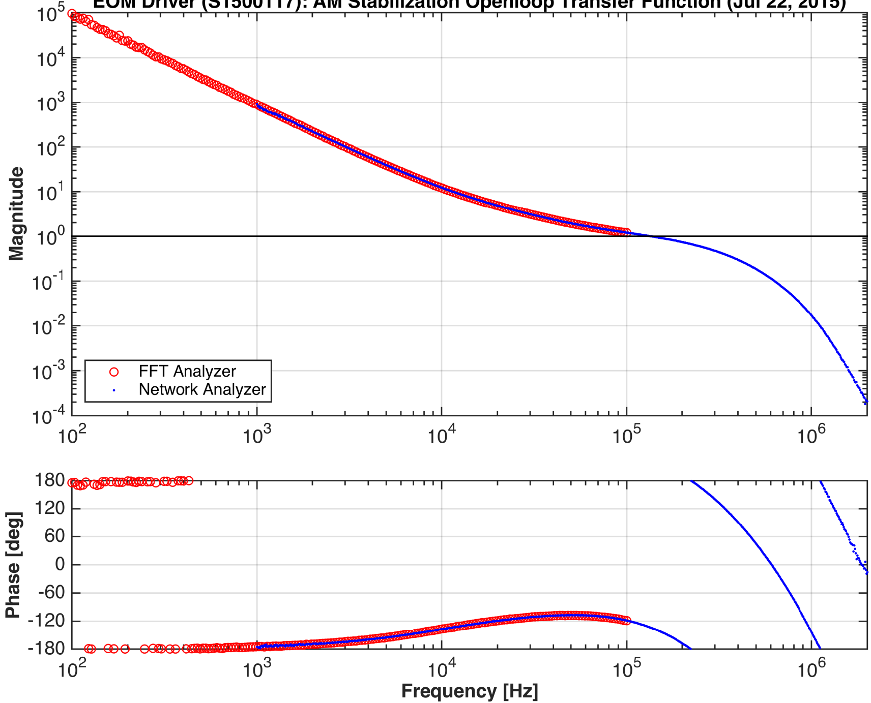
EOM Driver (S1500117): AM Stabilization Openloop Transfer Function (Jul 22, 2015)
