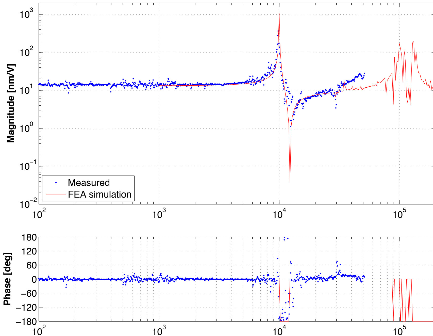
OMC PZT response: Comparison between measurement and FEA analysis (2014/9/8)
