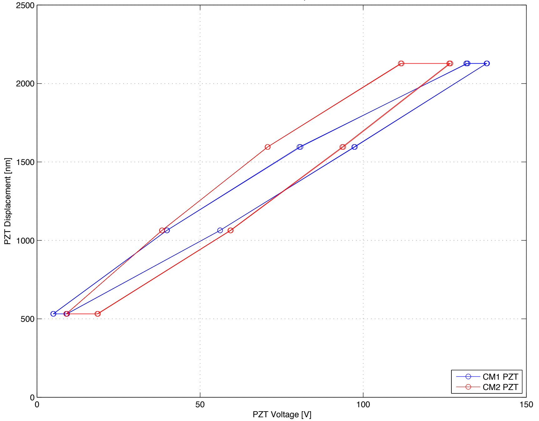
3rd OMC: PZT DC response test
