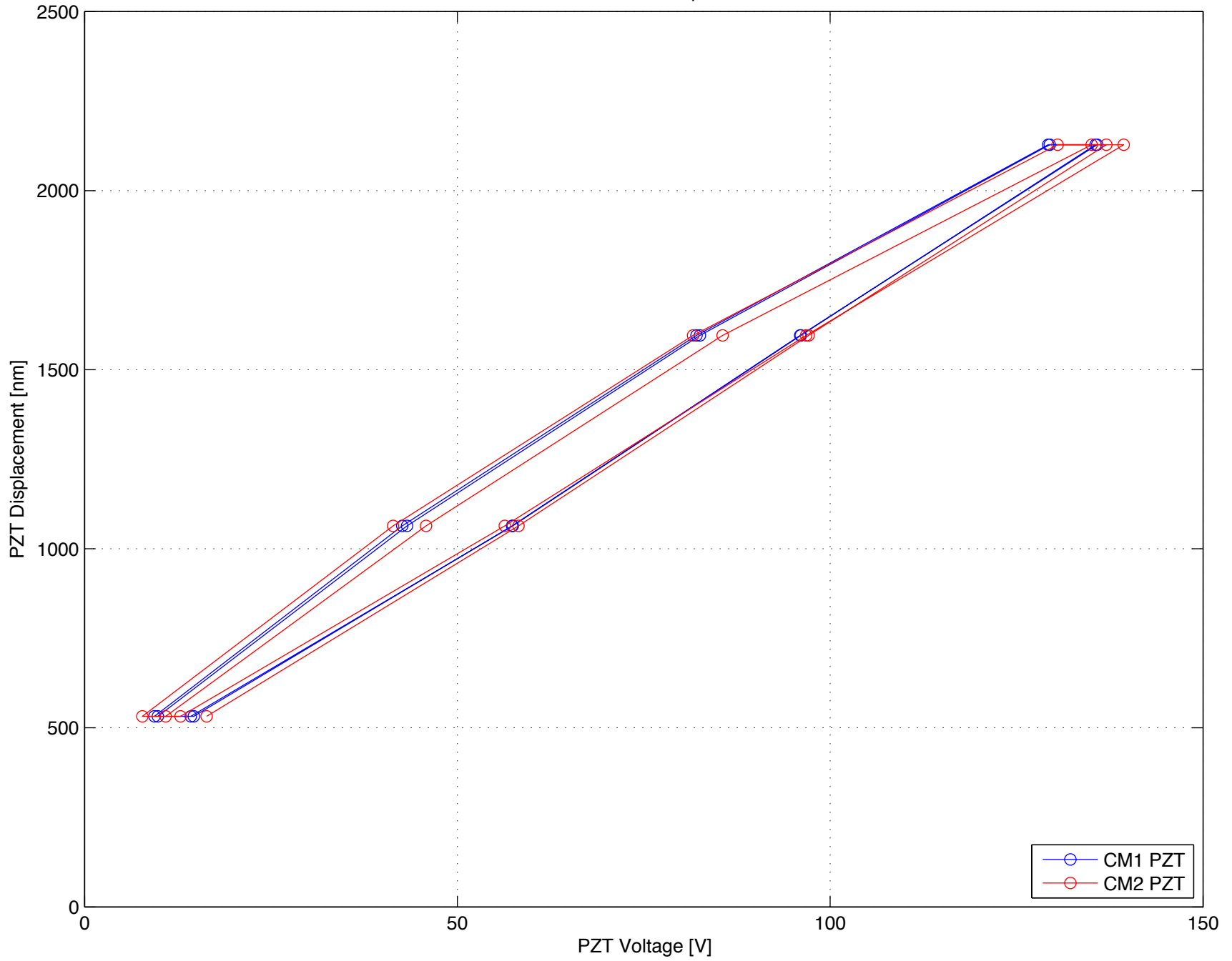
L1 OMC: PZT DC response test
