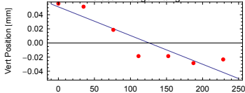
Vertical Wedge Fitting ~ A1
