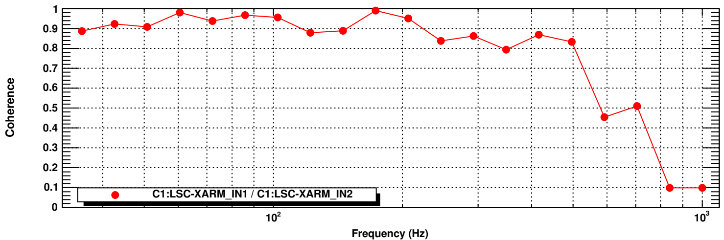
Coherence function
