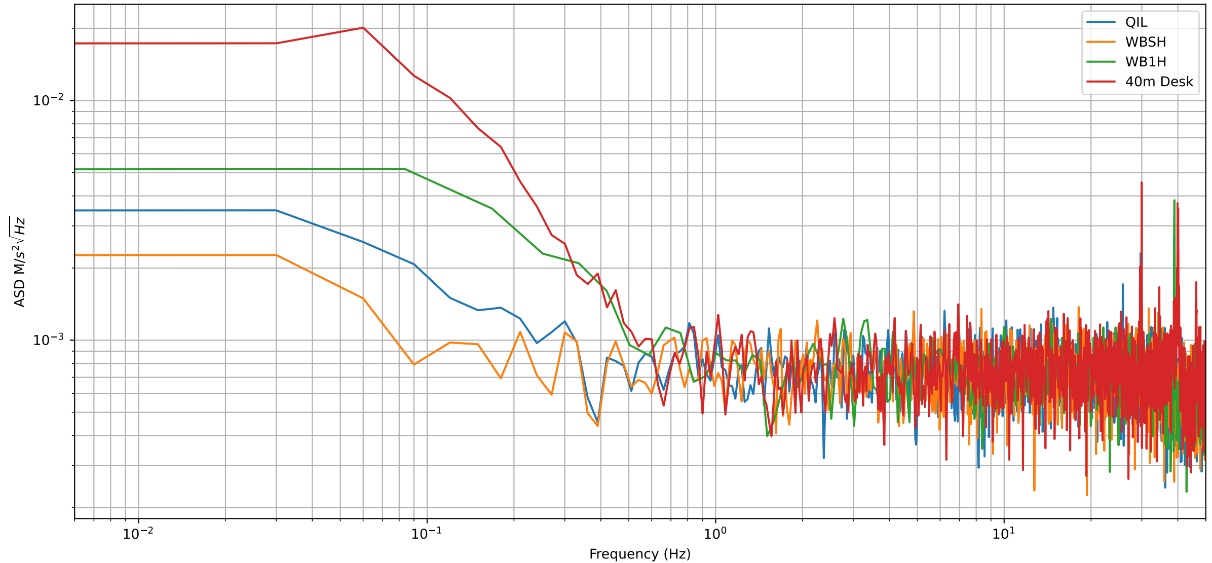
ASD Acceleration at Different Test sites
