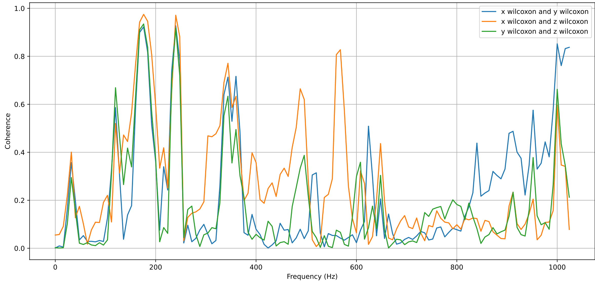
Coherence between different 40m sensors
