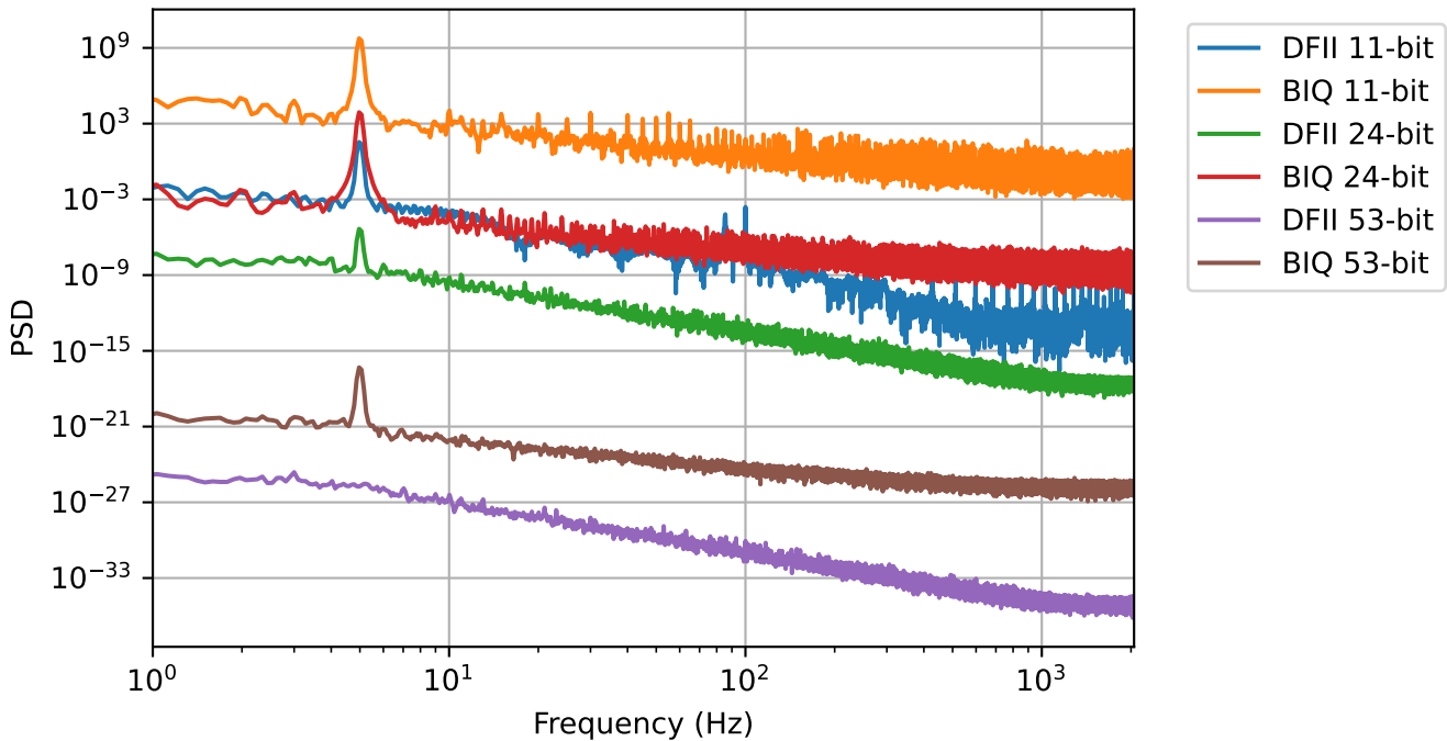
PSD of Quantization Noise for Dual-Sine Input
