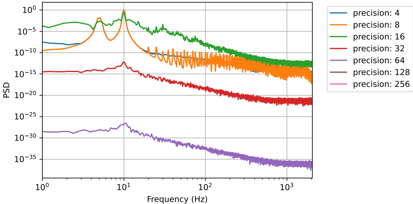
PSD of Quantization Noise for Dual-Sine Input
