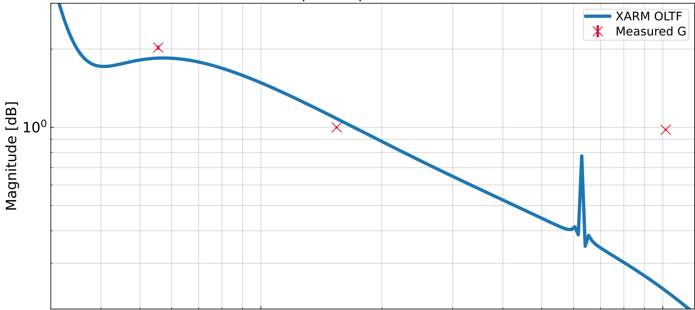
XARM Open Loop Transfer Functions
