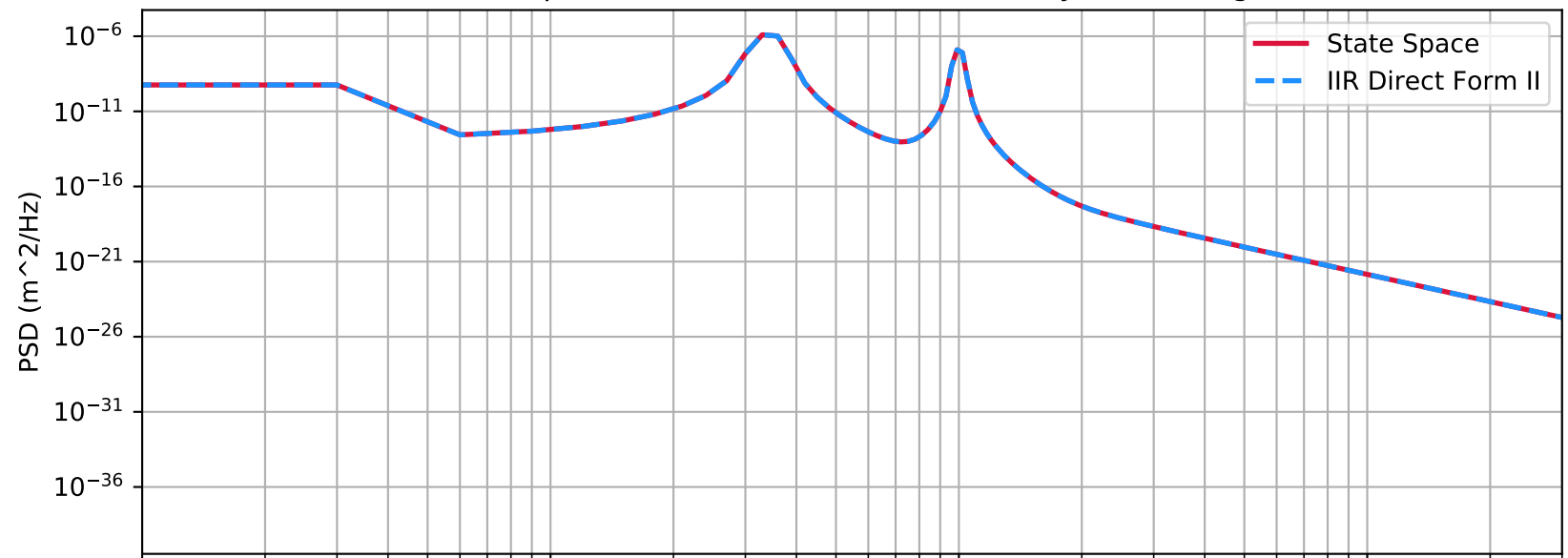
PSD comparison of 64-bit models driven by 3.42Hz Signal
