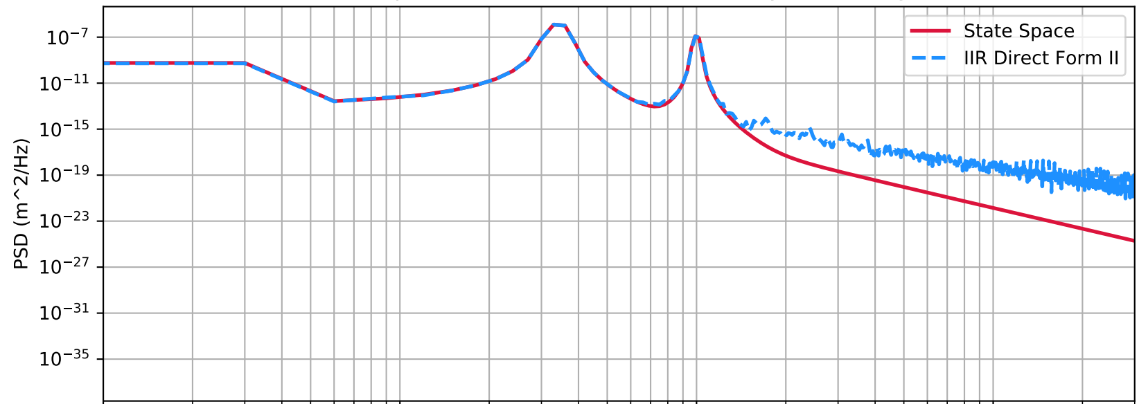
PSD comparison of 32-bit models driven by 3.42Hz Signal
