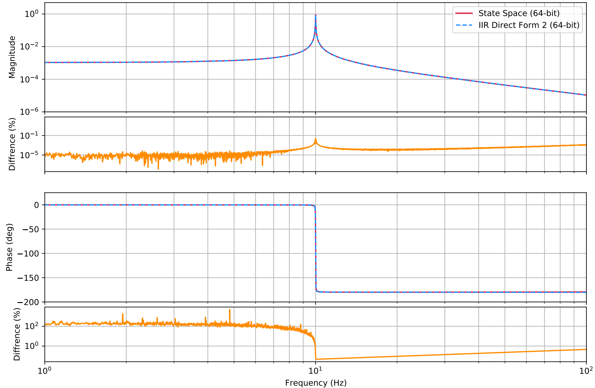
Transfer Function of State Space and IIR Filter of Suspension
