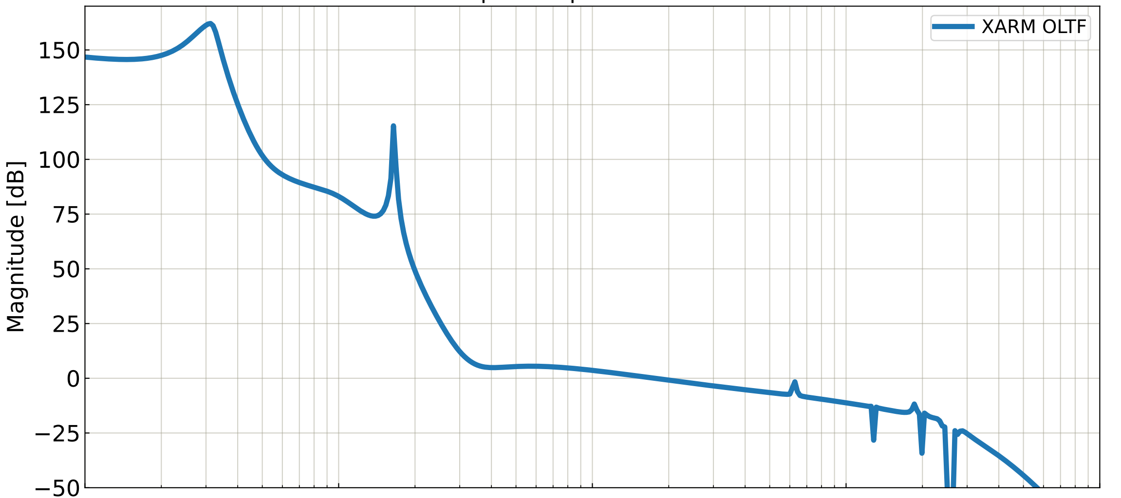
XARM Open Loop Transfer Functions
