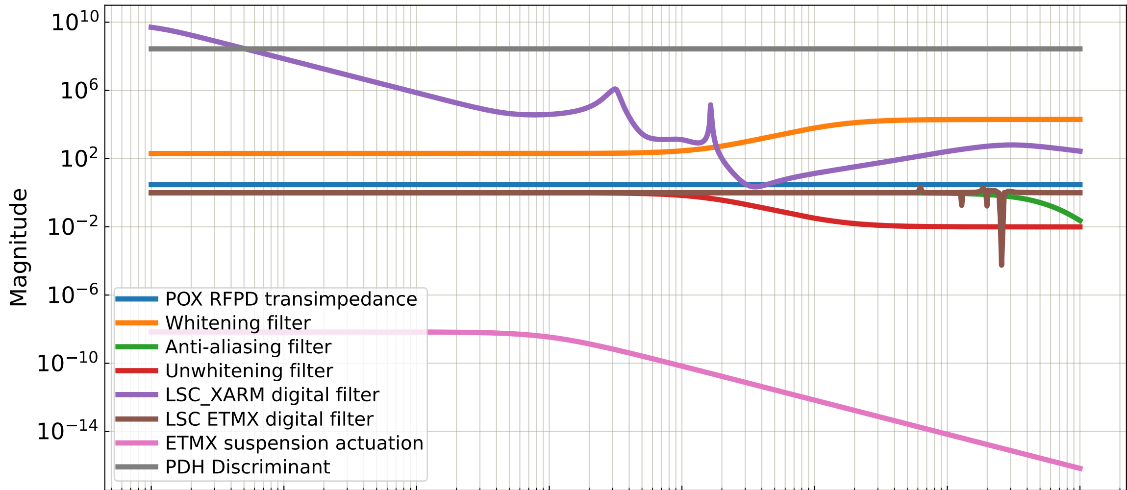
XARM POX Lock Model Transfer Functions
