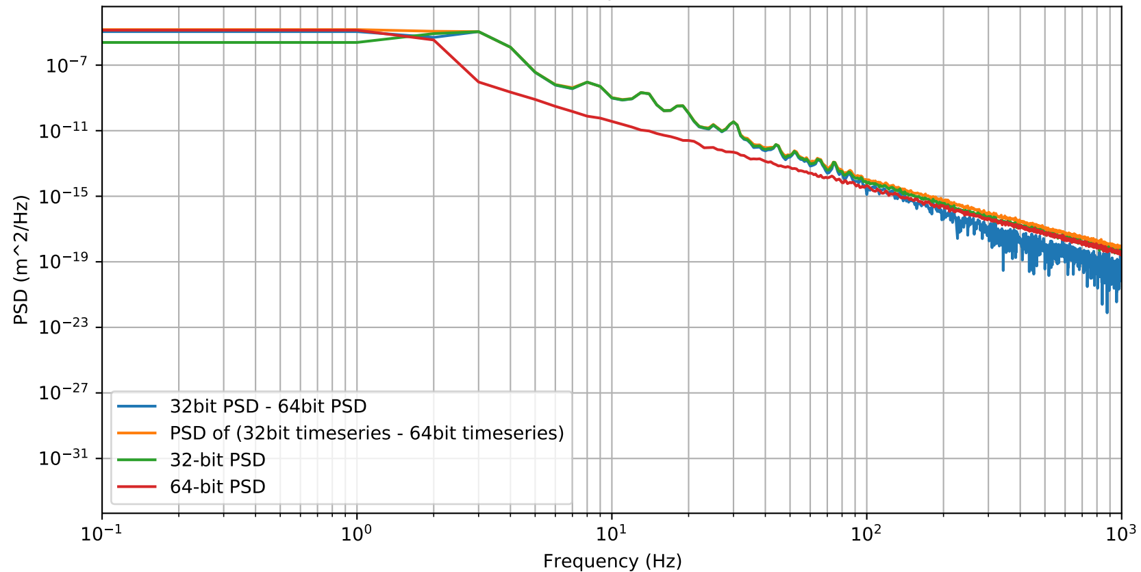
Noise Spectrum
