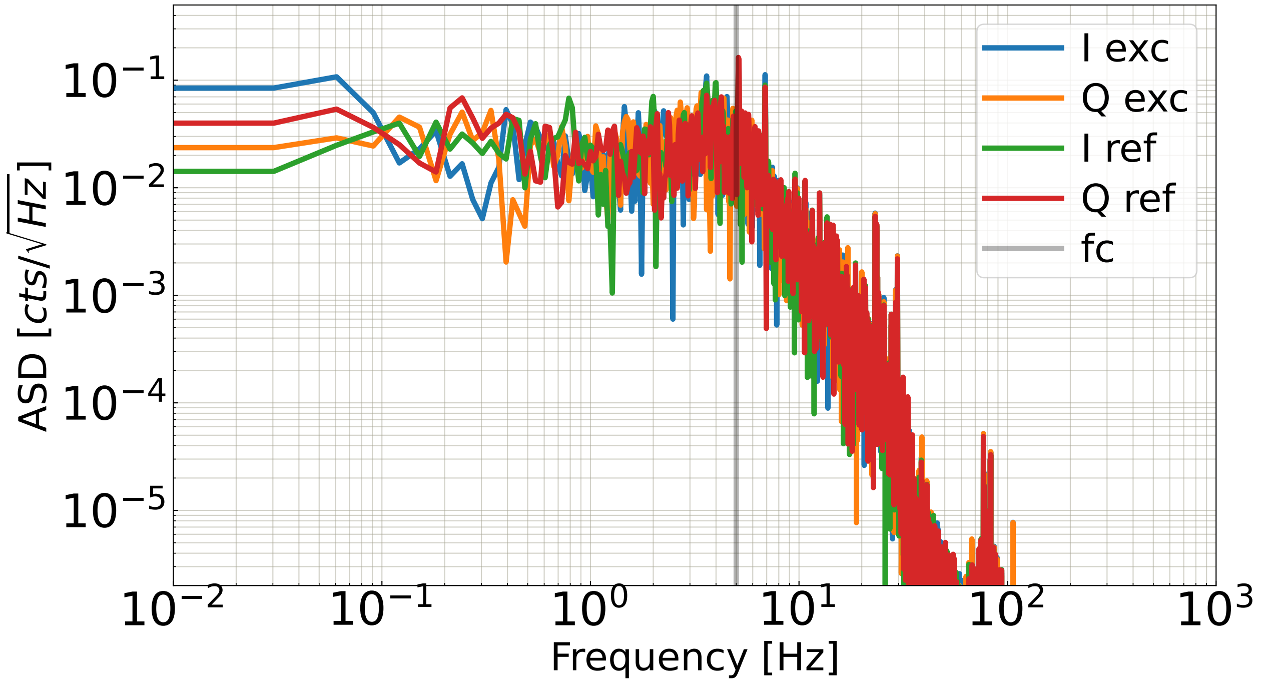
Demodulated ASD
