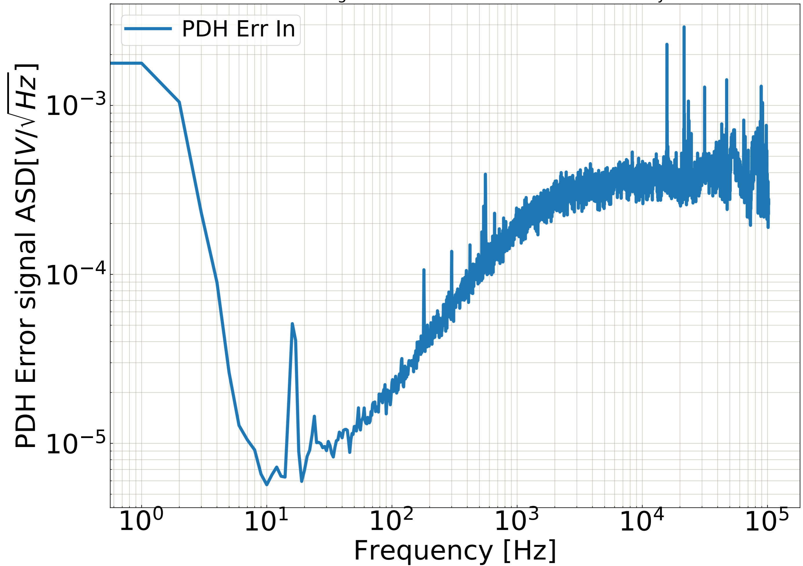
PDH Error signal ASD for Xend Green Laser with Arm cavity
