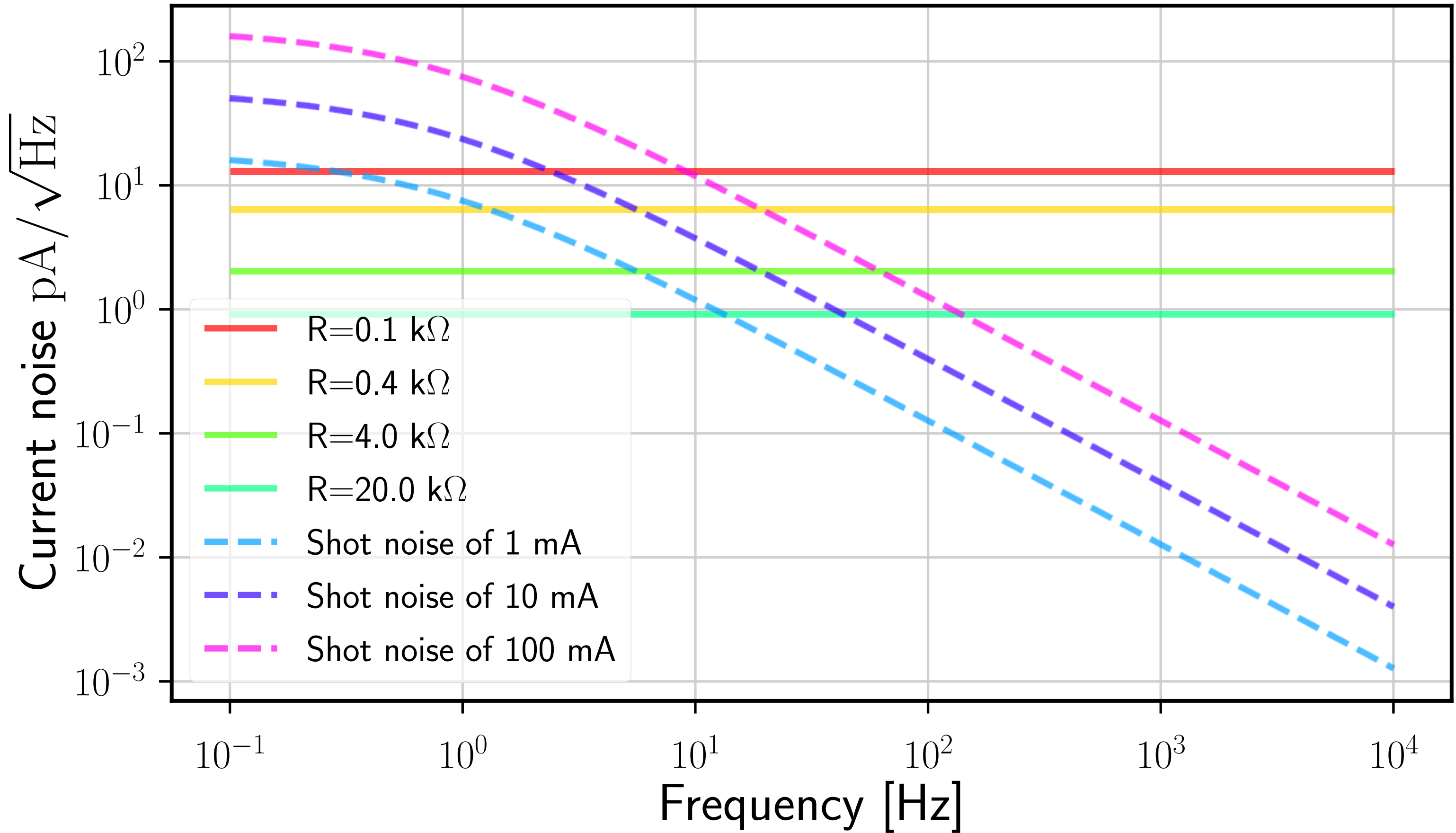
Relative contribution of shot noise and Johnson noise for coil driver (single channel)
