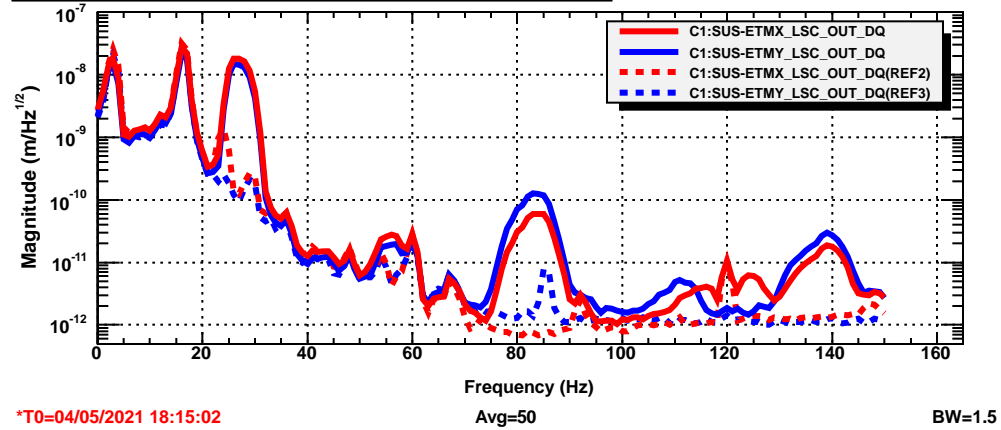
Effect of Noise Injection at Arm Locking Control Signals
