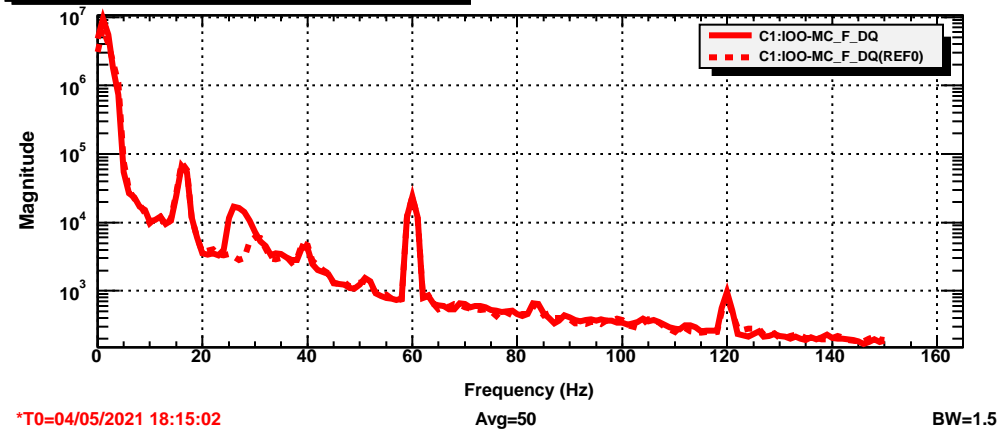
Effect of noise on IMC resonant frequency
