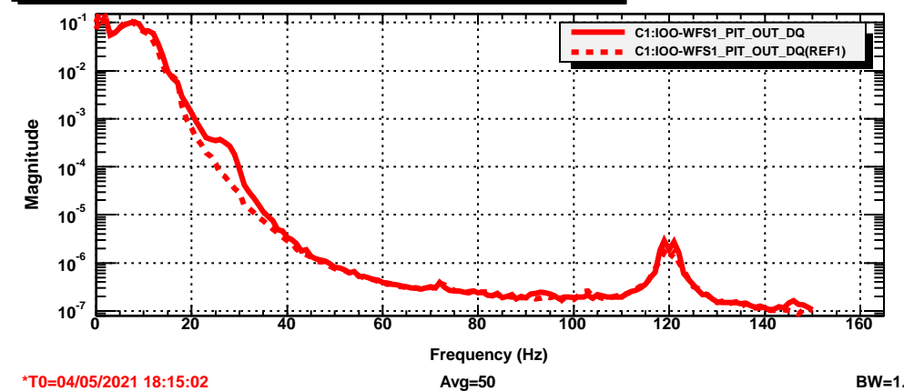
Suppression of noise by WFS loop (just before injection point)
