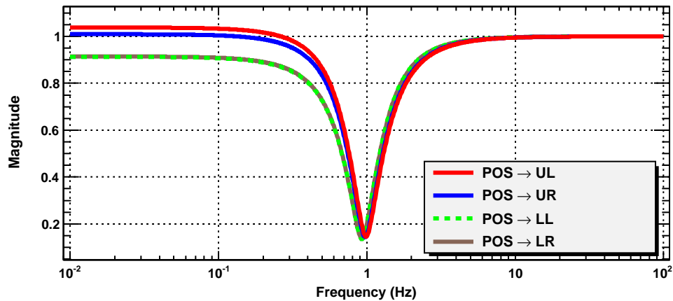
MC2 POS F2A Filters with Q = 7
