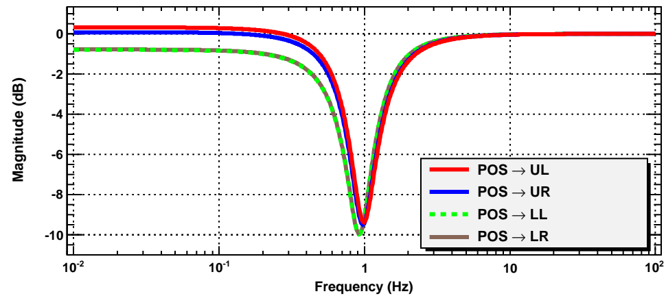
MC2 POS F2A Filters with Q = 3
