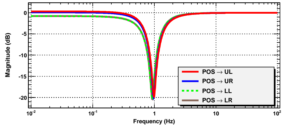
MC2 POS F2A Filters with Q = 10
