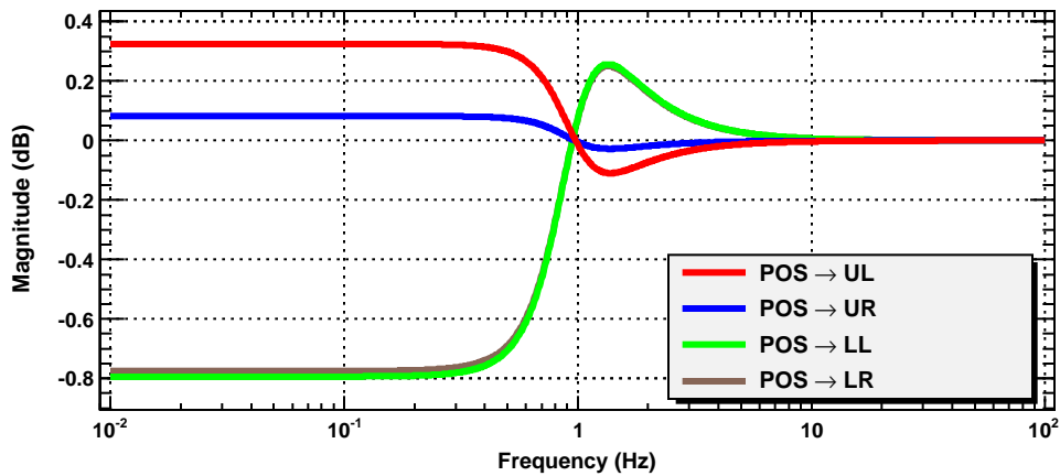
MC2 POS F2A Filters (Nominal Q = \sqrt{G\_DC} )
