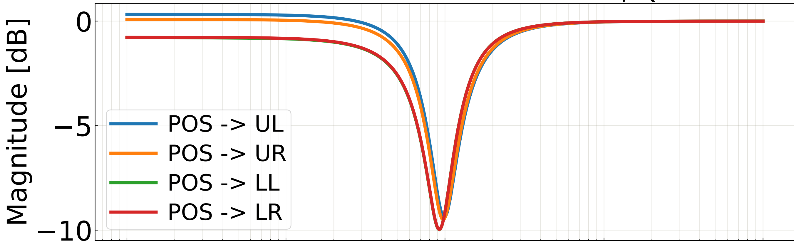
MC2 Filter banks for POS column, Q = 3
