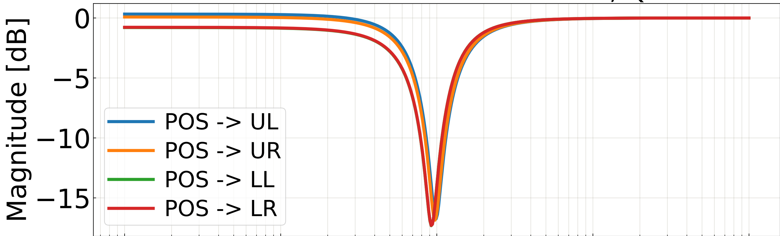
MC2 Filter banks for POS column, Q = 7
