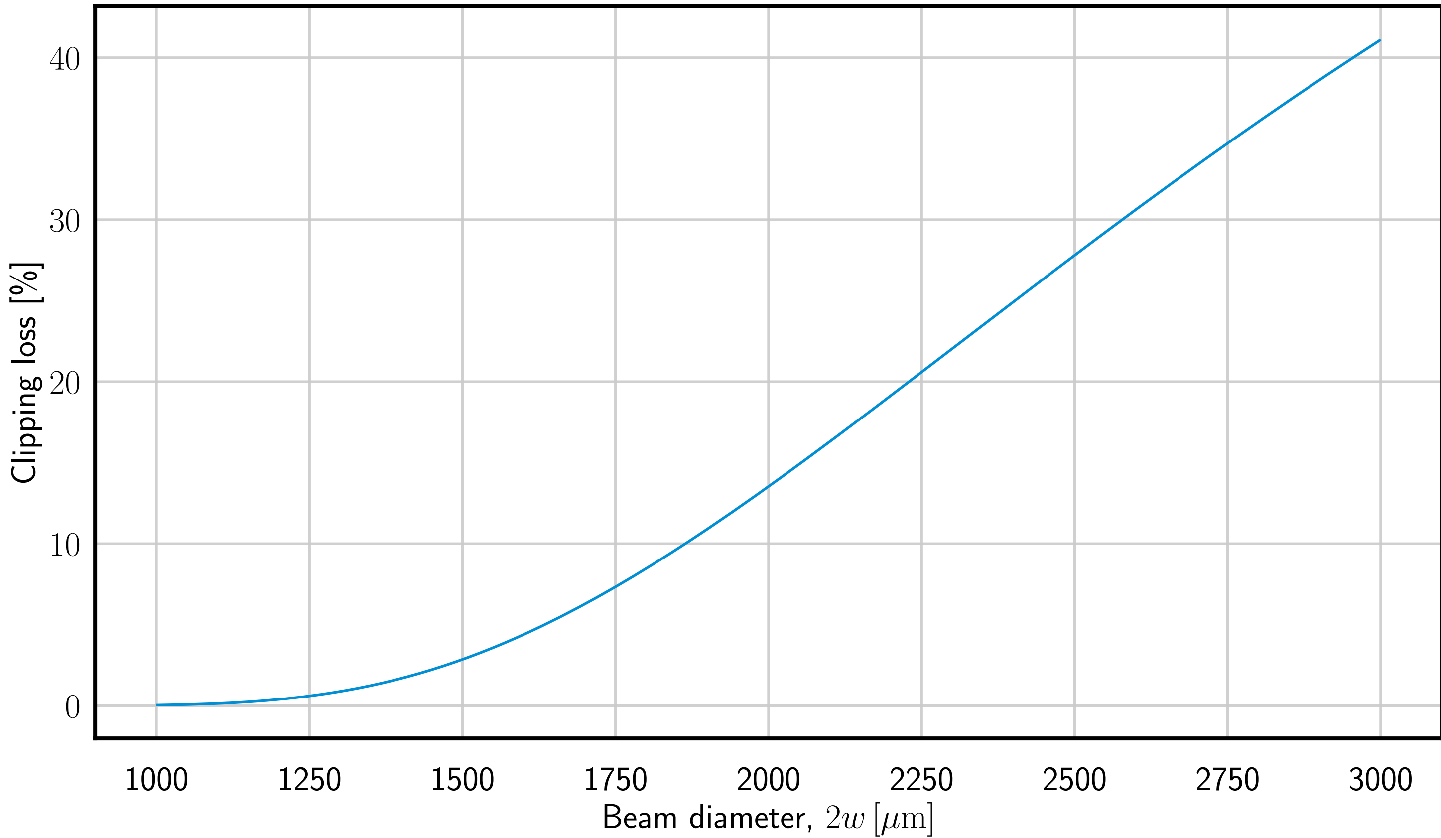
Clipping loss due to finite EOM aperture size
