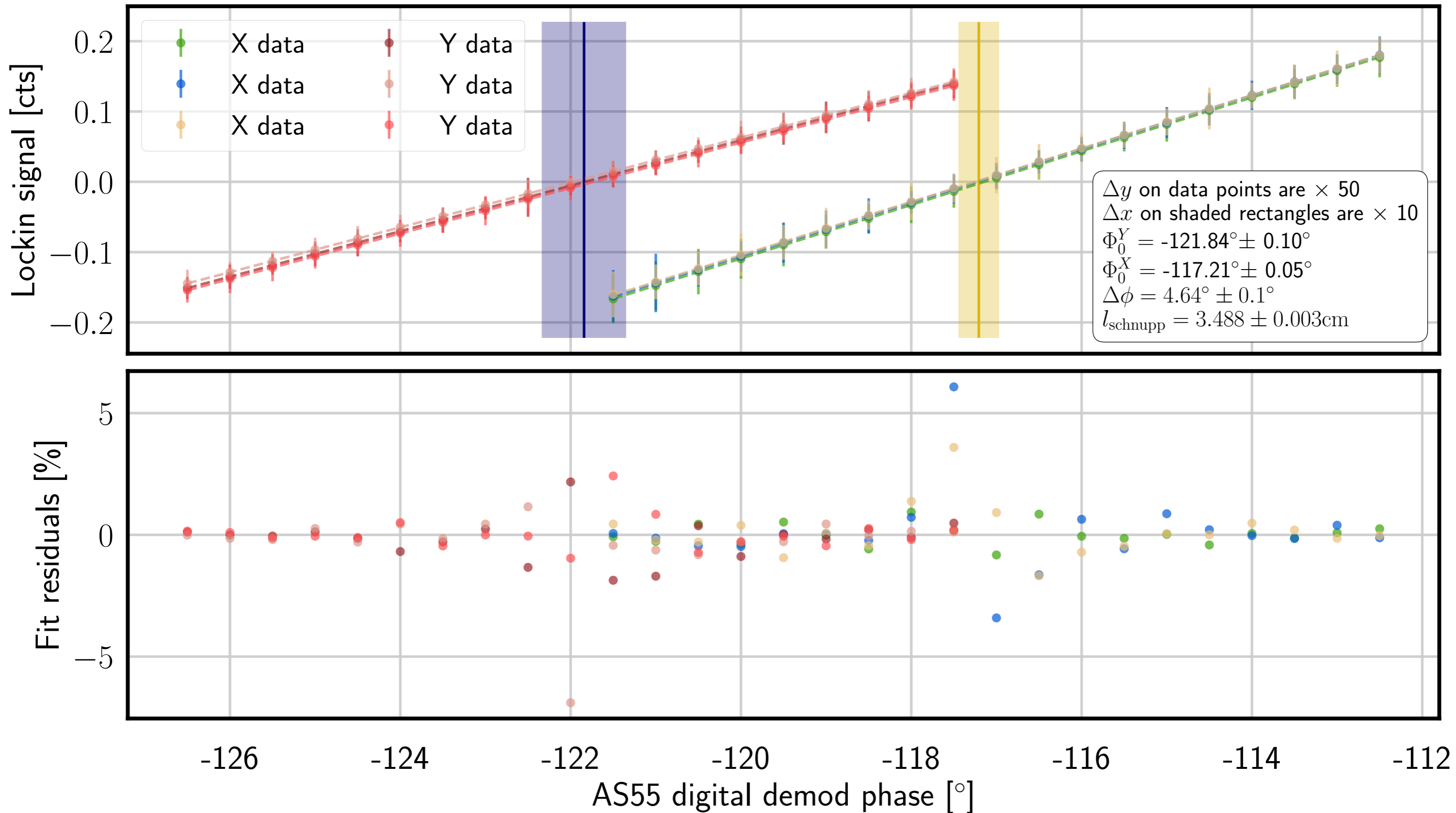
Determining Schnupp asymmetry by detecting phase of 55 MHz field in single arm lock
