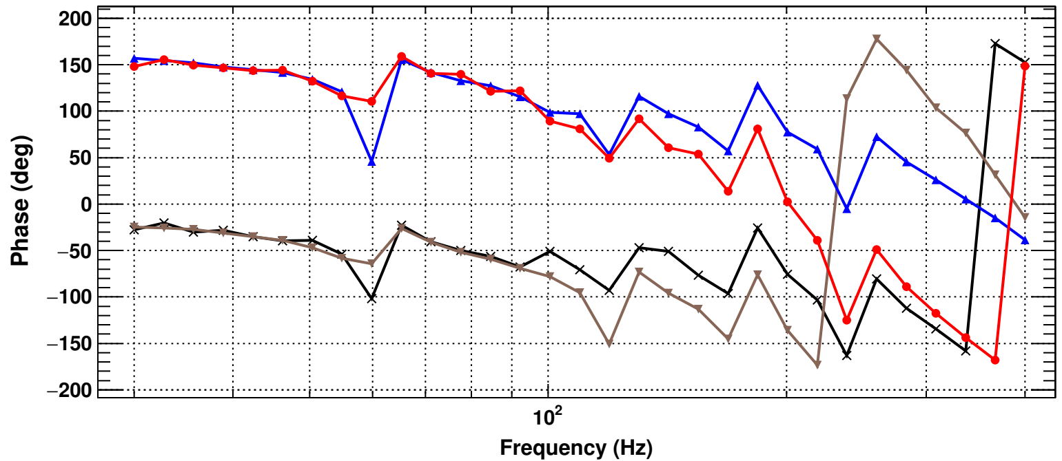
Transfer function
