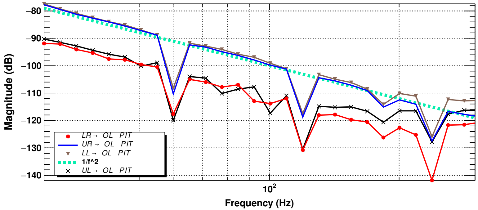
Transfer function
