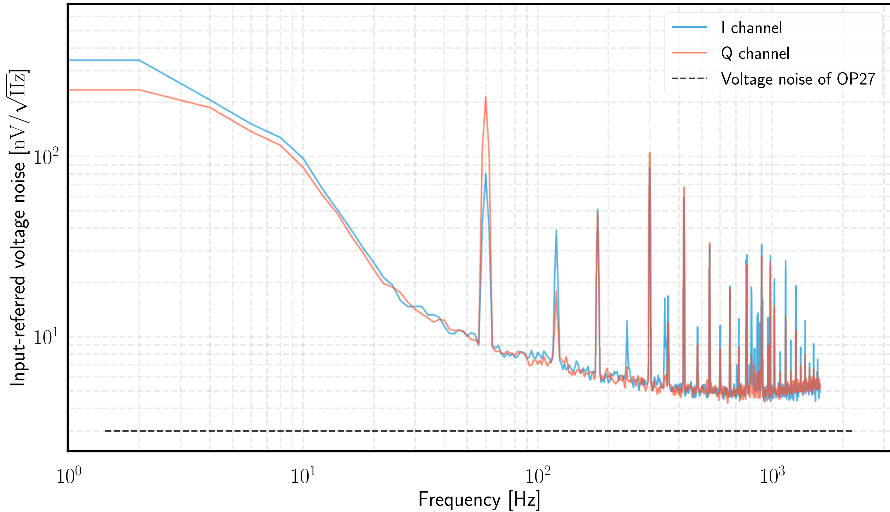
Measured noise of REFL55 demod board (PD input terminated, LO input driven at +3dBm)
