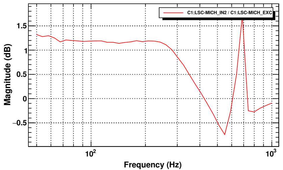
MICH Closed Loop Gain
