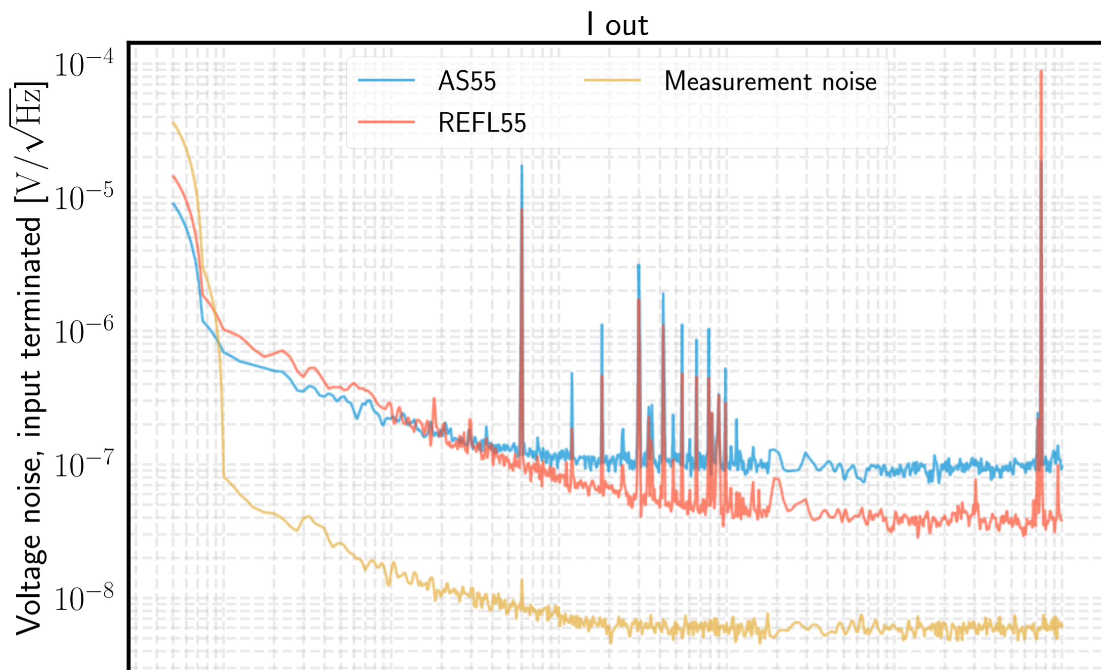
D990511 Demod board noise, with D040179 preamp installed
