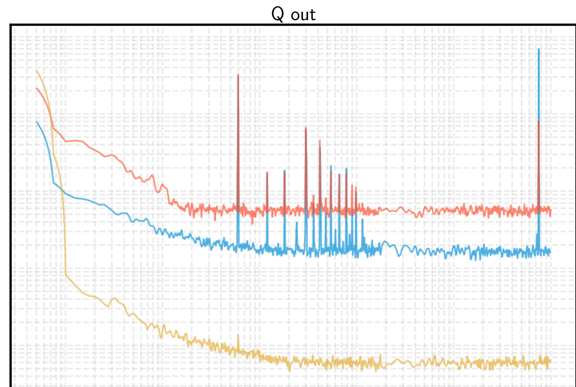
D990511 Demod board noise, with D040179 preamp installed
