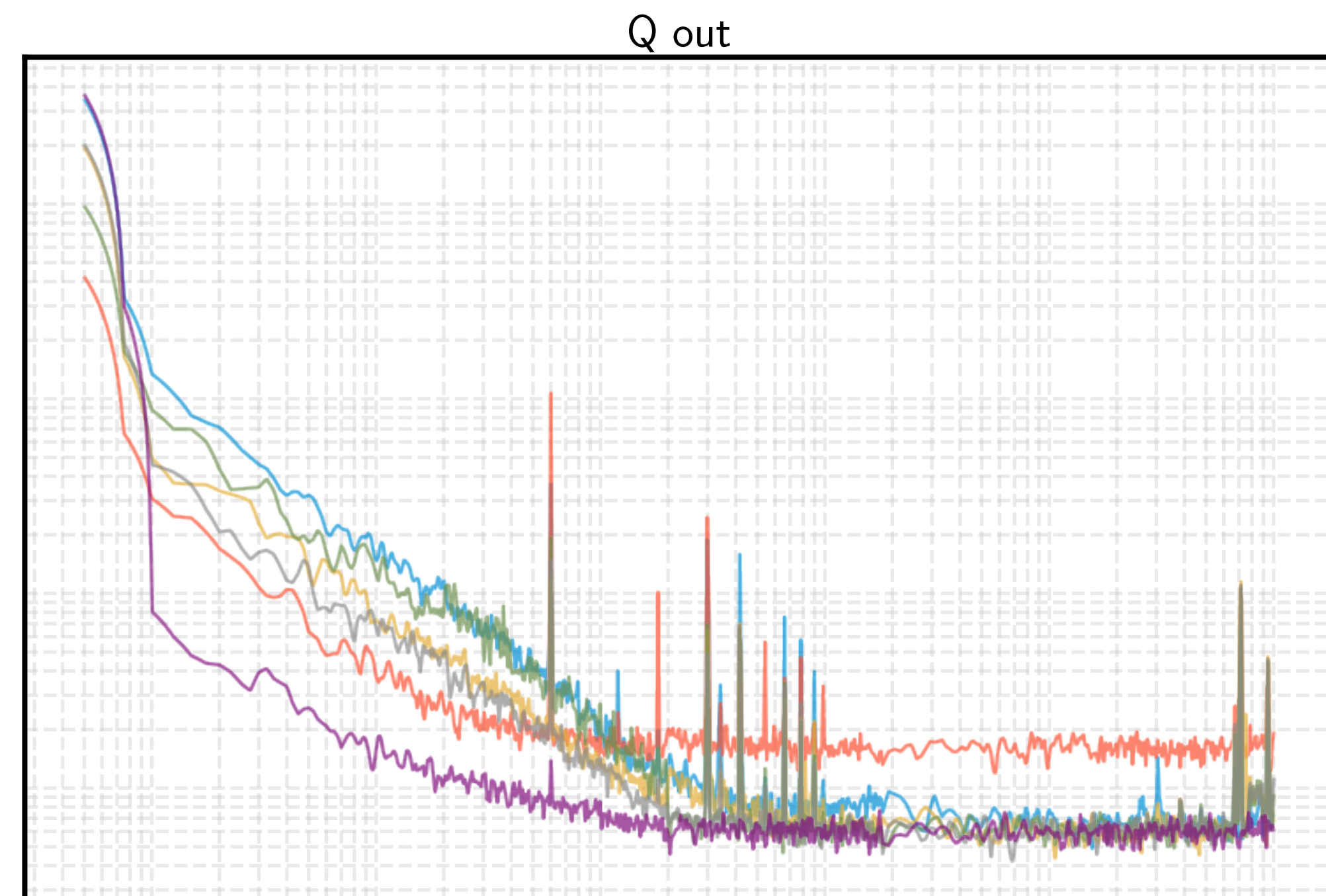
D990511 Demod board noise, without D040179 preamp installed
