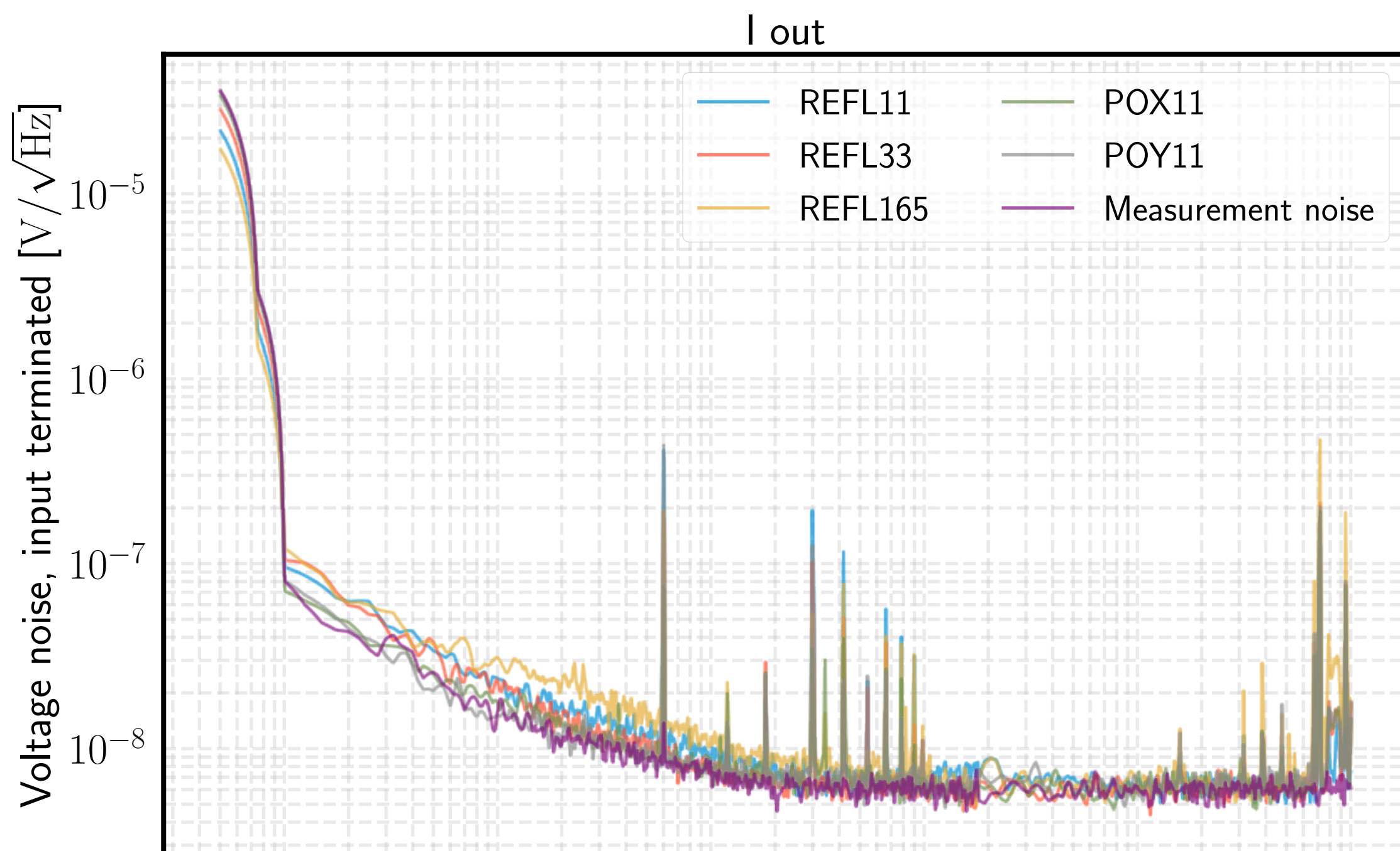
D990511 Demod board noise, without D040179 preamp installed
