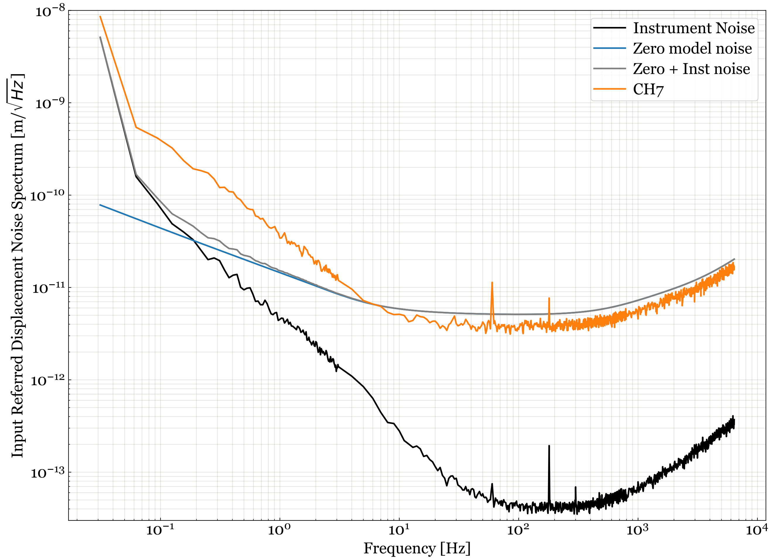
D11000687 S2100029 Input Referred Displacement Noise Spectrum.
