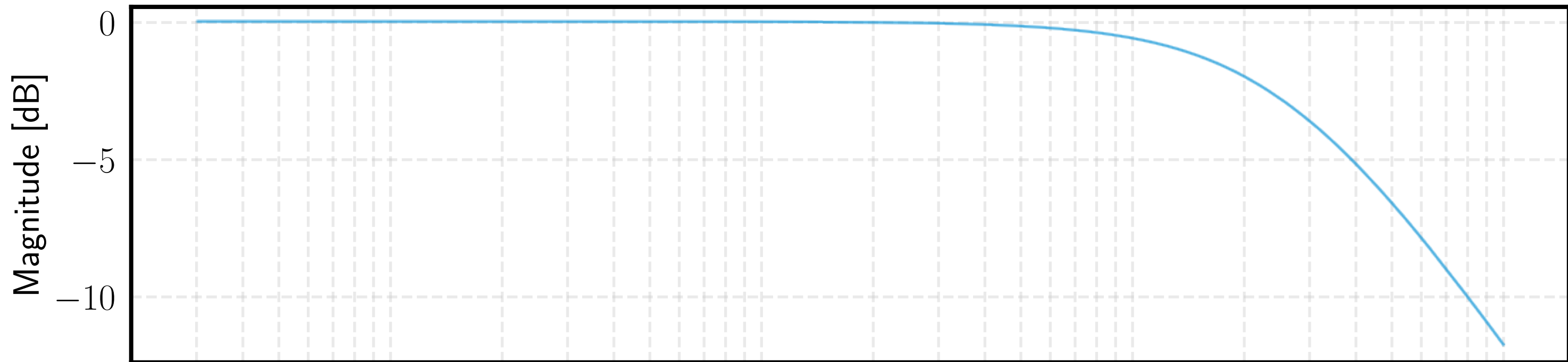
Transfer function of Differential Receiving Input Stage (J1 to TP2)
