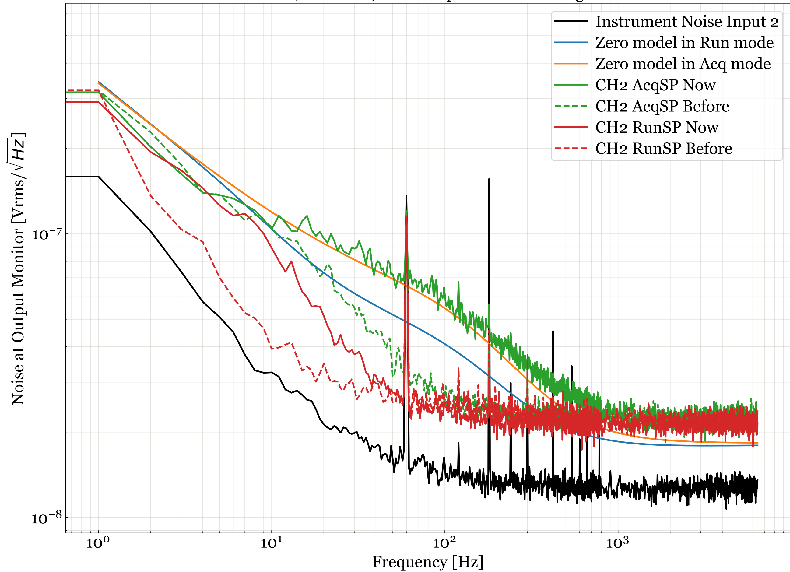
D11000687 S2100027 CH2 Output Monitor Voltage Noise
