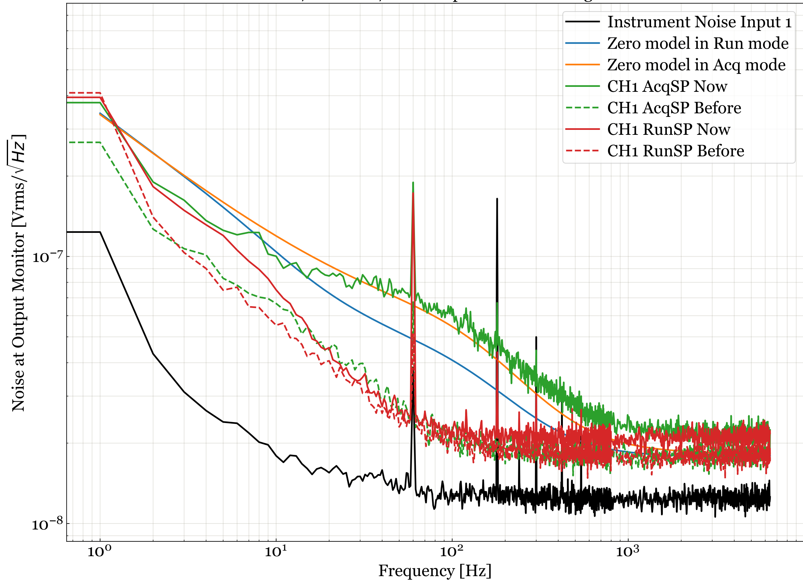
D11000687 S2100027 CH1 Output Monitor Voltage Noise
