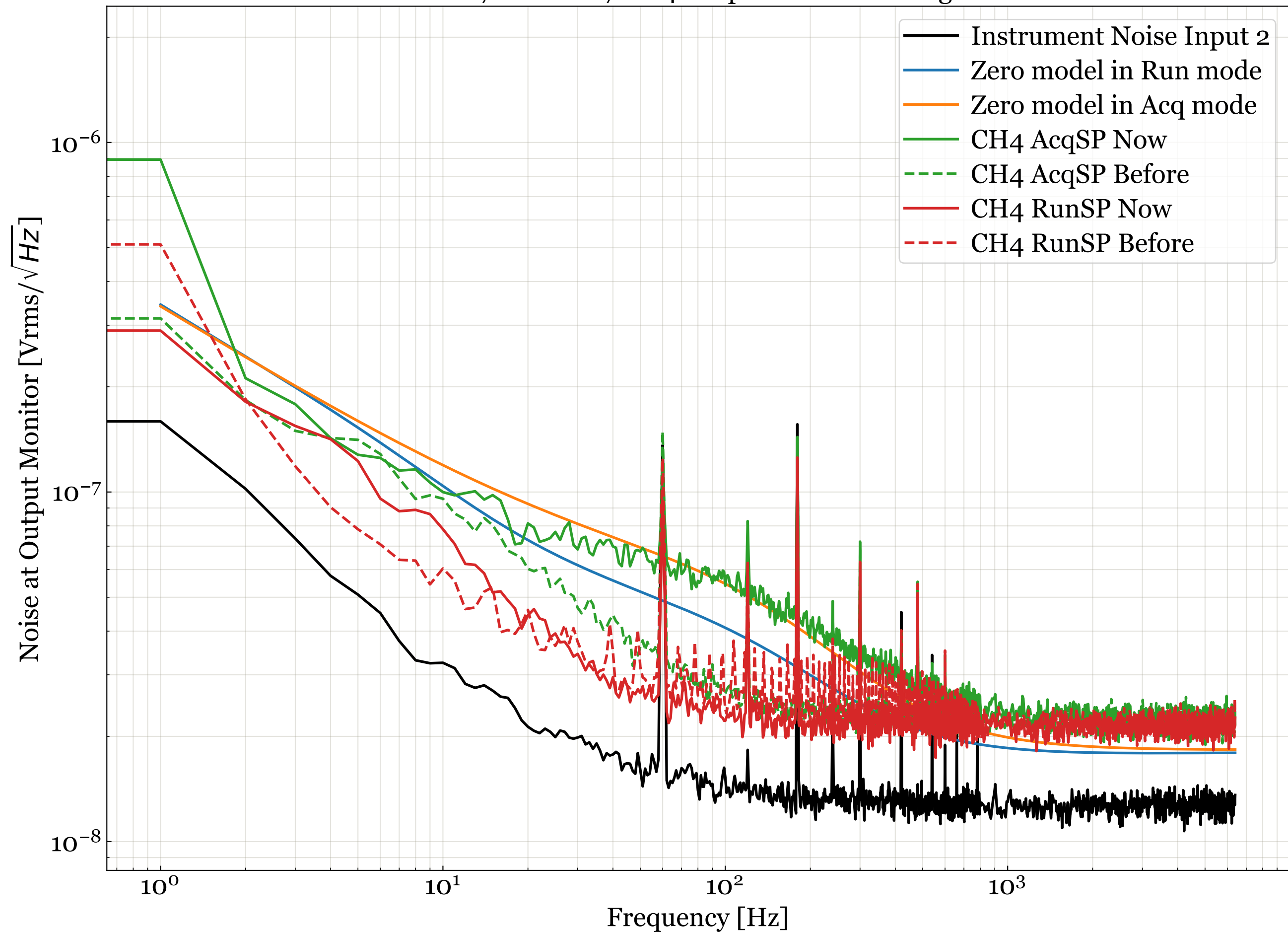
D11000687 S2100027 CH 4 Output Monitor Voltage Noise
