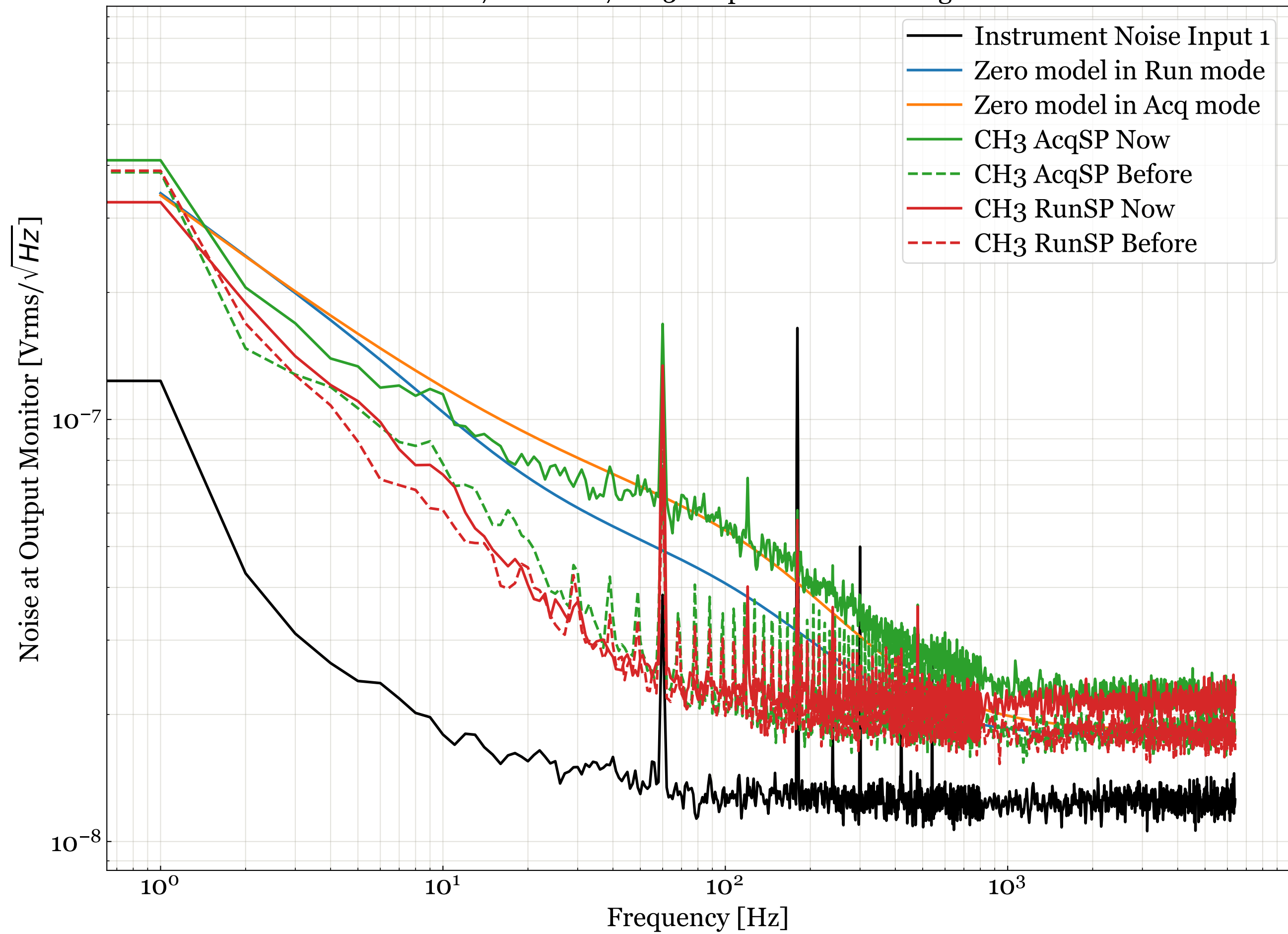
D11000687 S2100027 CH3 Output Monitor Voltage Noise
